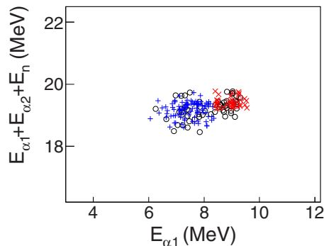
FIG. 7. Reconstructed sum \alpha + \alpha + n energy versus the energy of an individual \alpha particle detected in MAGNEX. Data are designated with open circles, and simulation related with breakup and charge exchange—see text—with crosses (in blue) and \times s (in red), respectively. It should be noted that our experimental setup was optimized on breakup; therefore, the acceptance for the charge exchange reaction was small and only few events are observed for this reaction.
