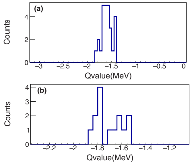
FIG. 9. Reconstructed Q -value spectra (a) with E_{\alpha 2} gate \geq 9.1 MeV and E_{\alpha 1} \leq 8.5 and (b) with E_{\alpha 2} gate \leq 9.1 MeV and E_{\alpha 1} \geq 8.5 . See also Figs. 1, 3, and 7.
