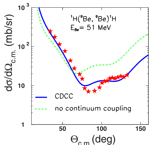
FIG. 6. elastic scattering angular distribution for {}^9\text{Be} + p at 51 MeV. Previous data [19,20], are compared with present CDCC calculations. Data statistical errors are included in the size of the symbols (see text).
