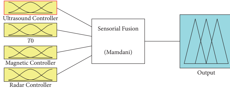
FIGURE 5: Structure of the fuzzy inference system.
