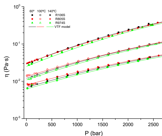
Figure 7. Pressure-viscosity curves for fumed silica suspensions for selected temperatures.
