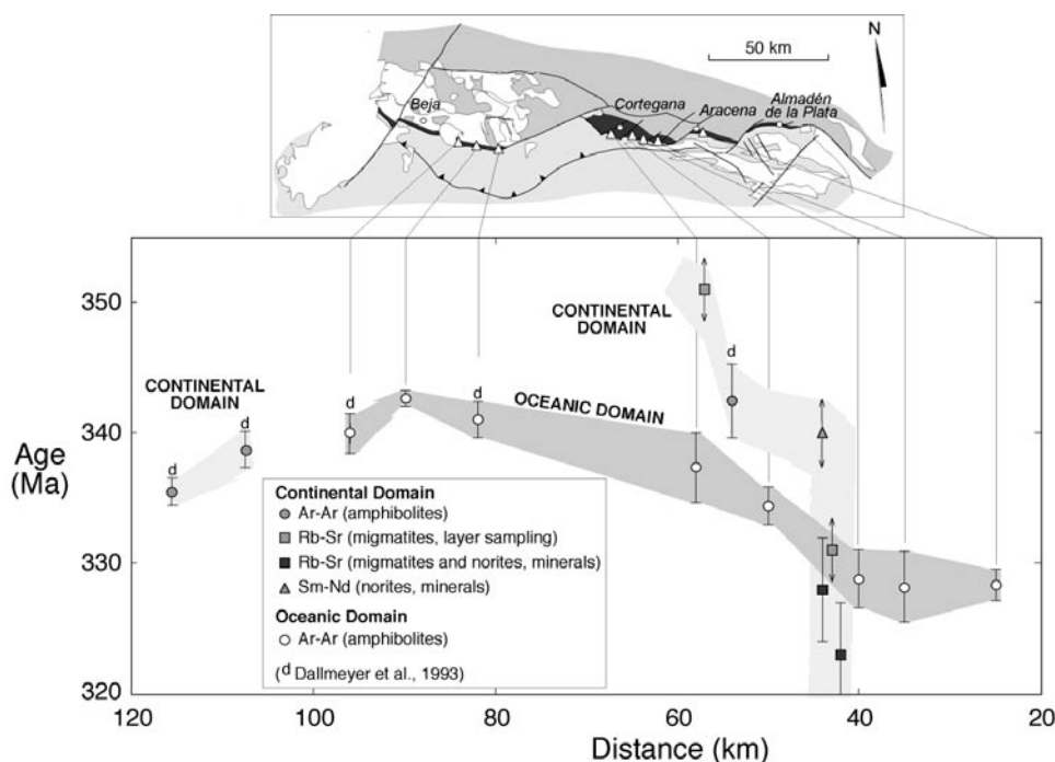
Fig. 14.- Variation of age of metamorphism with distance along the Acebuches metabasites, discarding the effect of displacements by late faults. The origin is arbitrarily located in Almadén de la Plata. Ages obtained in the rocks of the CD are also shown. The arrows are indicative of larger error bars (from Castro et al. , 1999a).
