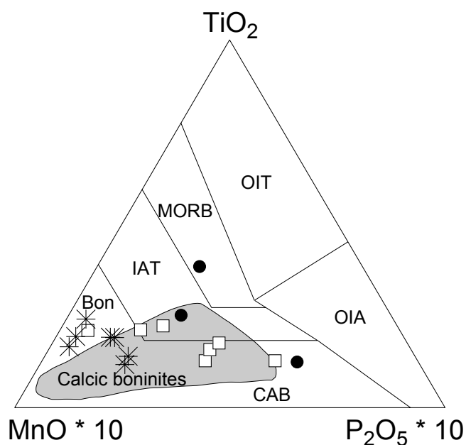
Fig. 13.- Representation of cumulated norites (asterisks), non-cumulated norites (squares) and dioritoids (circles) from the AMB (El-Hmidi, 2000) in the triangular TiO 2 -MnO * 10-P 2 O 5 * 10 diagram (Mullen, 1983). Fields are MORB (Mid Ocean Ridge Basalt), OIT (Ocean Island Tholeiite), OIA (Ocean Arc Alkali basalt), CAB (island-arc Calc-Alkaline Basalt), IAT (Island-Arc Tholeiite) and Bon (Boninite). The shaded area encloses representative analyses of calcic boninites from the Troodos complex in Cyprus (Rogers et al. , 1989), the Tonga trench in the Pacific Ocean (Falloon et al. , 1989) and the Vestfold Hills in the Antarctic shield (Kuhener, 1986).
