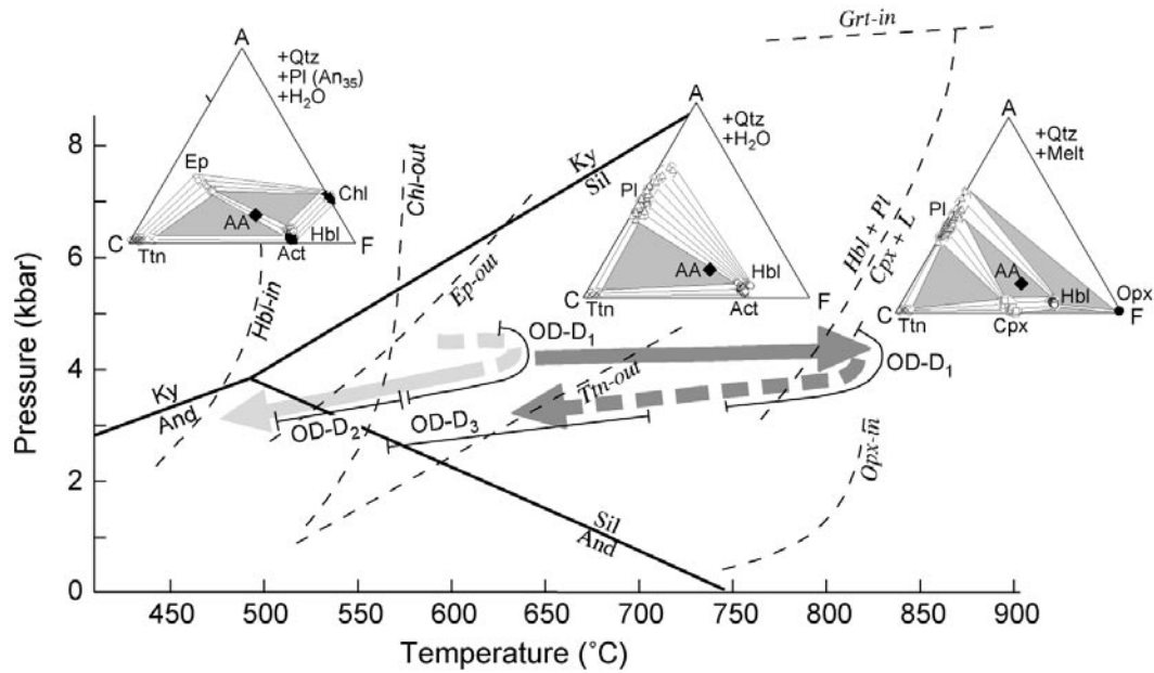
Fig. 6.- P-T-d paths deduced for the Acebuches metabasites: banded amphibolites with clinopyroxene (dark path) and mafic schists (light path). Solid lines correspond to paths deduced directly from observed mineral assemblages whereas dashed lines correspond to paths inferred by indirect observations. ACF diagrams showing the mineral assemblages corresponding to the three main metamorphic zones described across the Acebuches metabasite series. a) The upper levels of the sheet belong to the clinopyroxene zone. b) Most of the series are amphibolites with a typical Pl-Hb assemblage. c) The mafic schists from the lower levels display a Pl-Hb-Act-Ep-Chl mineral assemblage.
