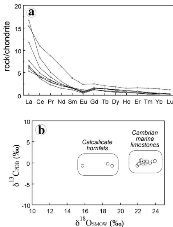
Fig. 10.- REE patterns (a) and isotopic ratios (b) of representative calcitic marbles from the Aroche sector.
