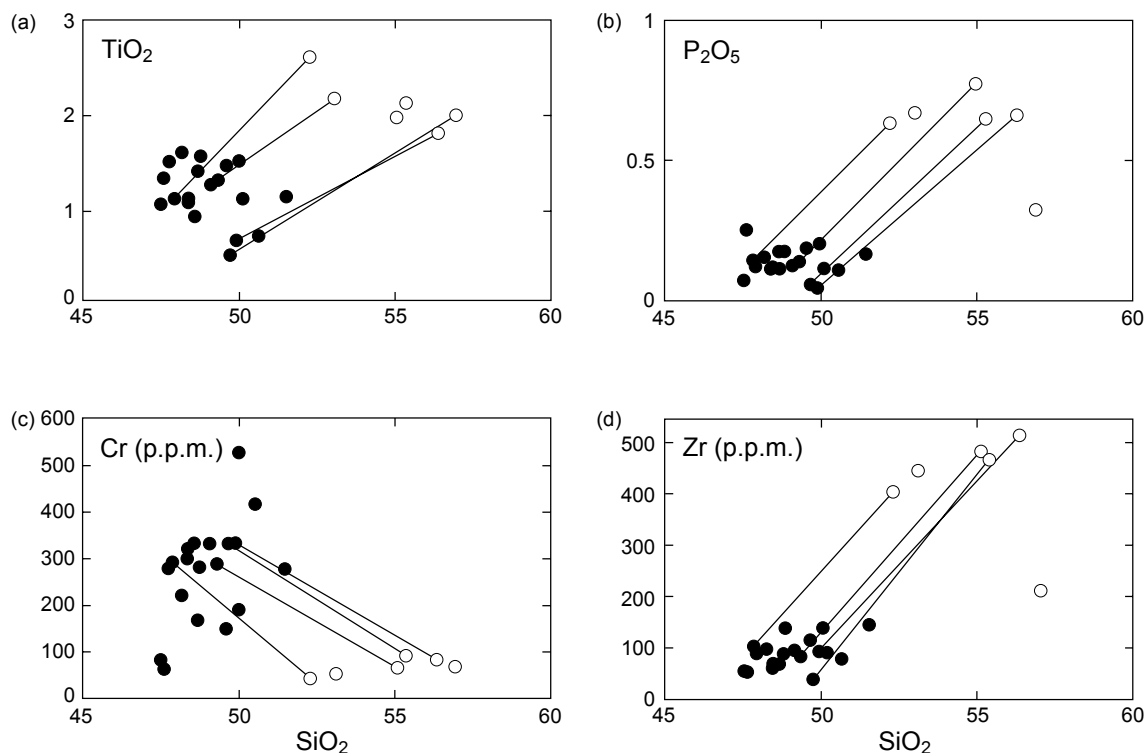
Fig. 12.- Silica variation plots for major and trace elements, showing the relationships between Pl-Hb and quartz-rich amphibolites from the Acebuches series. Tie-lines link pairs of samples from two adjacent layers (from Castro et al. , 1996b).
