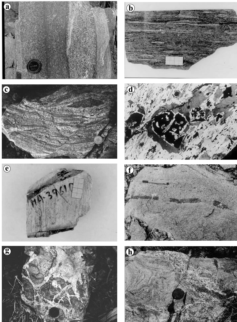
Fig. 2.- Photographs of different rock types found in the AMB. a) Coarse-grained banded amphibolites of the OD with alternating light coarse grained, grey medium grained and dark fine-grained bands. b) Mafic schists from the Acebuches metabasite series showing, on the mylonitic foliation planes, a penetrative stretching lineation. c) Stromatic migmatites of the CD, with a layering defined by alternating leucosome and melanosome layers. Also, paleosome bodies are observed at the top of the photograph. d) Kinzigitic gneisses of the CD. Skeletal blast of hercynite surrounded by a plagioclase rim. The matrix is constituted by dynamically recrystallised cordierite along with fibrolite aggregates. e) Leptinitic gneiss of the CD with a penetrative mylonitic foliation defined by pyroxene and amphibole blasts. f) Marbles of the CD. The metamorphic foliation is defined by melanocratic blasts (marked by the pen) as well as by the calc-silicate boudins. The tabular shape of the boudins suggests that the calc-silicate layers are much more competent than the surrounding marble. g) Calc-silicate rocks of the CD with agmatic texture. h) Pegmatitic Pl-Hb body showing intrusive relationships with foliated and folded calc-silicate rocks.
