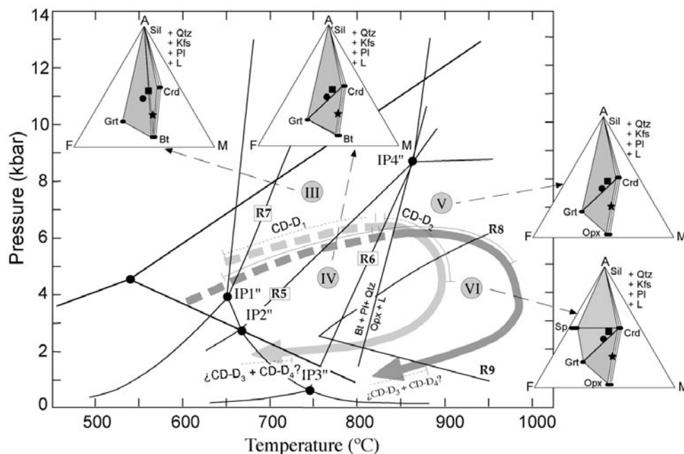
Fig. 9.- P-T-d paths deduced from petrography for Los Romeros migmatites, Los Molares nebulites and the charnockitic nebulites (light path), as well as for the kinzigitic gneisses (dark path) of the aluminous series of the CD (El-Biad, 2000; Díaz Azpiroz, 2001). Solid segments were deduced directly from observed textures, whereas dashed segments were inferred from indirect observations. Roman numbers indicate stability fields crossed by the deduced paths, which are characterised by their respective mineral assemblage represented in AFM diagrams. The black circle stands for the Los Romeros migmatites and the Los Molares nebulites whole rock composition (El-Biad, 2000). The black square stands for the kinzigitic gneiss whole rock composition (El-Biad, 2000) and the black star stands for the theoretical composition of the charnockitic nebulites.
