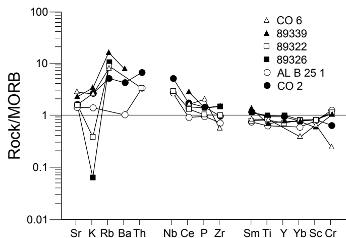
Fig. 11.- Rock/MORB normalised spider-diagrams with representative samples of the Acebuches metabasites (from Castro et al. , 1996b).
