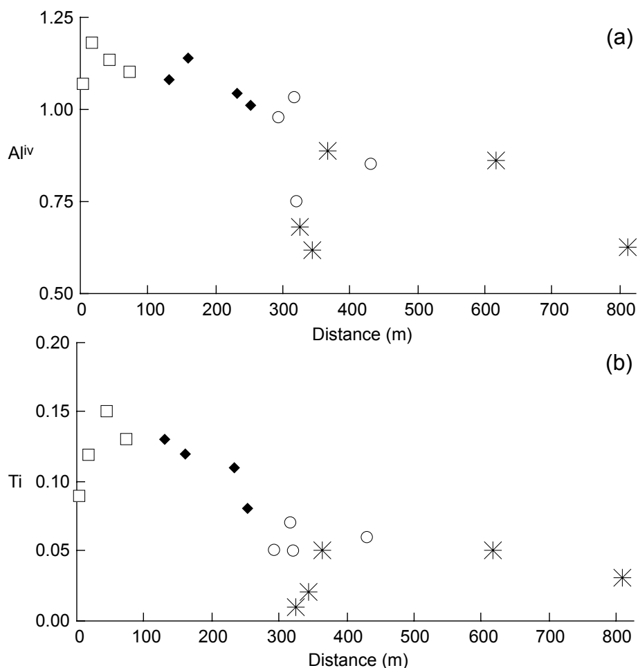
Fig. 7.- Evolution of the Al^{iv} (a) and Ti (b) in amphiboles from the Acebuches metabasites, with respect to the distance to the Calabazares shear zone (namely, the structural top of the series), in the Veredas cross-section (see figure 1b). Banded amphibolites with (open squares) and without (black rhombi) clinopyroxene, sheared amphibolites (open circles) and mafic schists (asterisks) are differentiated.
