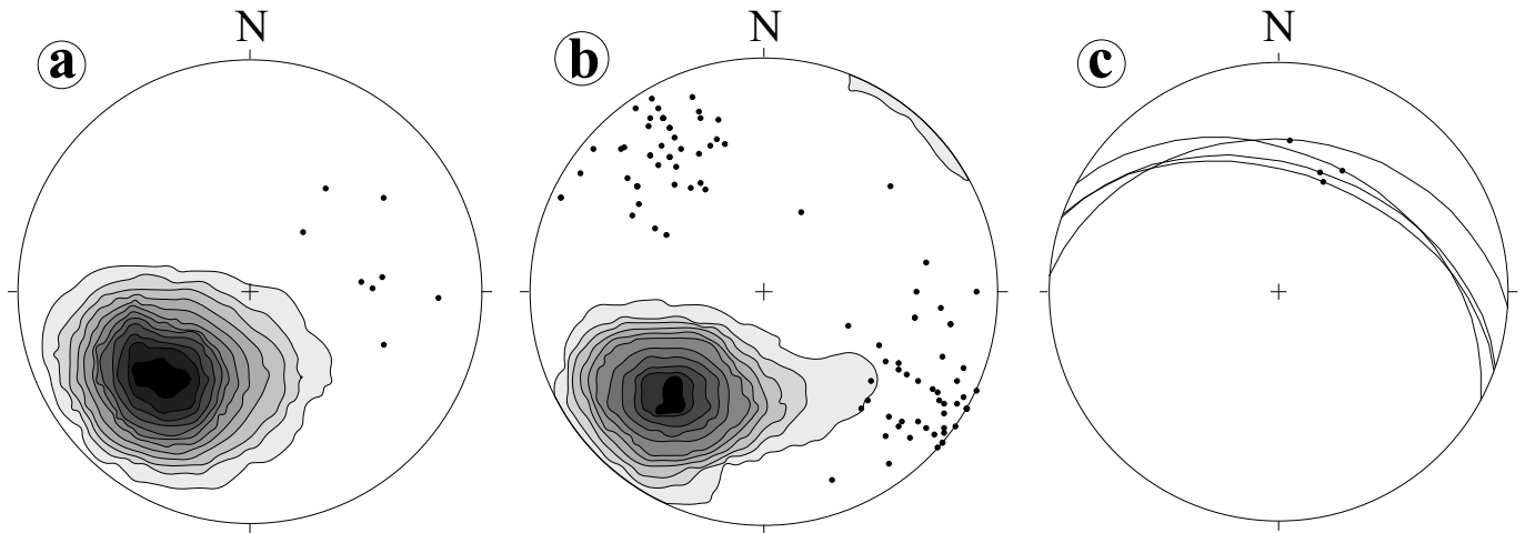
Fig. 3.- Lower-hemisphere, equal-area, projections of foliation and lineation data from the Acebuches metabasite series. Kamb contour and contour intervals are 2\sigma . a) OD-S 1 (98 poles to planes) and OD-L 1 (8 lines). b) OD-S 2 (205 poles to planes) and OD-L 2 (98 lines). c) OD-S 3 (4 planes) and OD-L 3 (4 lines).
