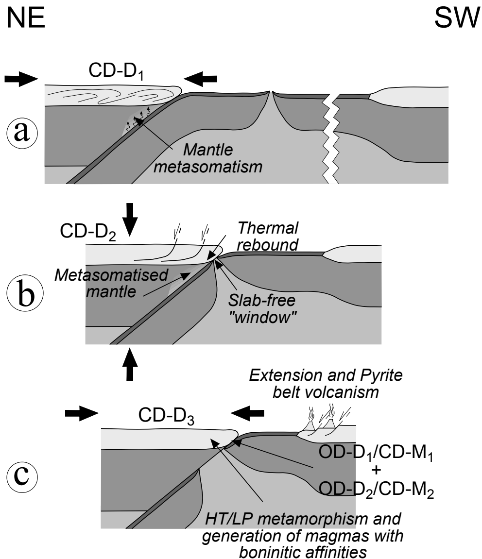
Fig. 15.- Tectonic model proposed for the variscan evolution of the AMB (simplified from Díaz Azpiroz et al. , 2003a). Geographic references are as in present (with no scales). a ) After the formation of an oceanic ridge between the Iberian autochthon and the allochthonous South-Portuguese plate, the oceanic leading plate is subducted beneath the Iberian plate. Metasomatism of part of the lithospheric mantle and CD-D 1 developed. b ) Subduction of the ridge as a consequence of the triple junction migration. The opening of a "slab-free window" gave place to a thermal rebound that heated up the base of the continental crust and produced magmas with boninitic affinities. At the same time extensional structures (CD-D 2 ) were generated. c ) Inverted HT/LP metamorphism and related shear deformation (OD-D 1 ) affecting the trailing oceanic plate. The accretion of the top of this plate to the base of the continental margin provoked the migration of the subduction plane to the SISZ. The continental margin, together with the Acebuches metabasites, overthrust the rest of the oceanic plate as well as the accretionary prism through the SISZ (OD-D 2 ). In the CD, upright folds generated (CD-D 3 ).
