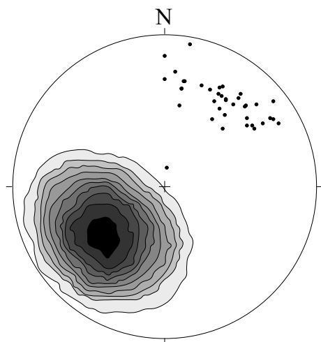
Fig. 5.- Lower-hemisphere, equal-area projection of poles to the CD-S 4 mylonitic foliation and the associated CD-L 4 stretching lineation (59 data). Kamb contours and contours are 2σ.
