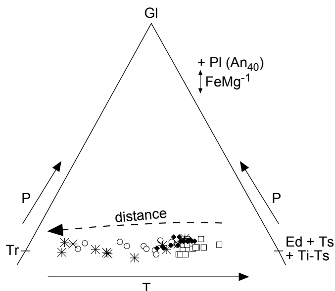
Fig. 8.- Qualitative thermobarometer (based on Castro et al. , 1996b) defined by a baricentric projection of amphiboles in the space Tr – Gl – Ed + Ts + Ti-Ts, through the \text{FeMg}^{-1} interchange and from \text{Pl}(\text{An}_{40}) . The curve marks the compositional evolution (with respect to the distance to the Calabazares shear zone) of the Acebuches amphiboles (symbols as in figure 7).
