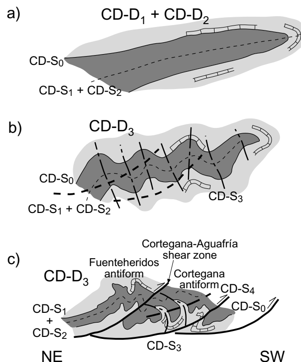
Fig. 4.- Schematic tectonic evolution proposed for the CD of the AMB (Díaz Azpiroz, 2001). a) As the result of the CD-D 1 and CD-D 2 deformation phases, km-scale recumbent folds and a high-temperature penetrative foliation (CD-S 2 ) were generated. b) CD-D 3 gave place to open symmetric upright folds. The discontinuous lines represent the localisation of the CD-D 4 shear zones. c) CD-D 4 produced km-scale thrusts, with a very penetrative mylonitic foliation (CD-S 4 ), and thrust accommodation folds (namely, the Fuenteheridos and the Cortegana antiforms).
