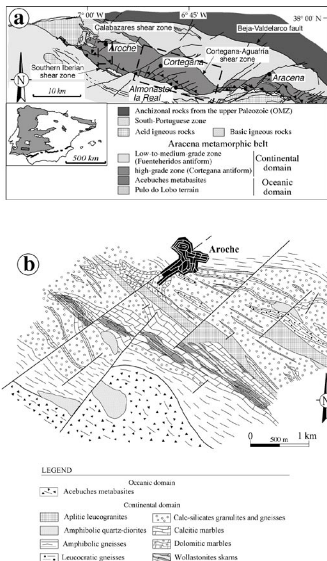
Fig. 1 (a and b).- a) The Aracena metamorphic belt (AMB) is located at the contact between the Ossa Morena and the South Portuguese zones of the Iberian Massif. Its trend (WNW-ESE) is parallel to the main structures of the Ossa-Morena Zone. The insets show detailed geological maps of the two areas considered in the present study. b) A small area of the contact between the oceanic and the continental domains (OD and CD, respectively) located to the south of Aroche.
