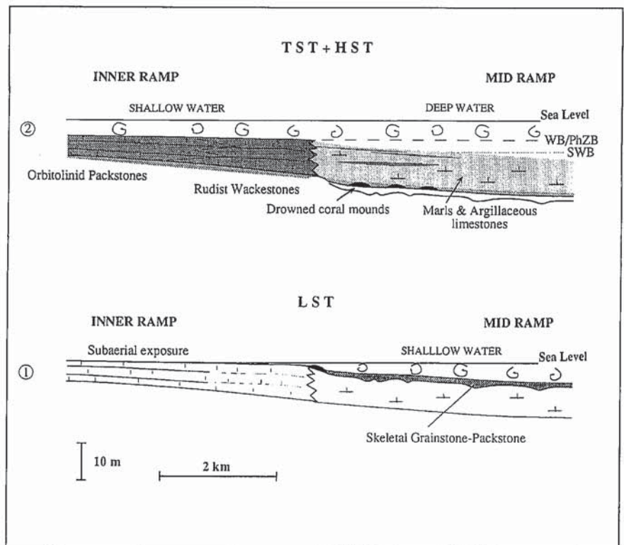
Fig. 5.- Ramp constructional dynamics and relative sea level. Note different sea level trends when shallow marine deposition occurs on the inner ramp (sea level tends to fall) and on the mid ramp (sea level tends to rise). Note also contrasting shallow marine sediments for inner and mid ramp settings.
