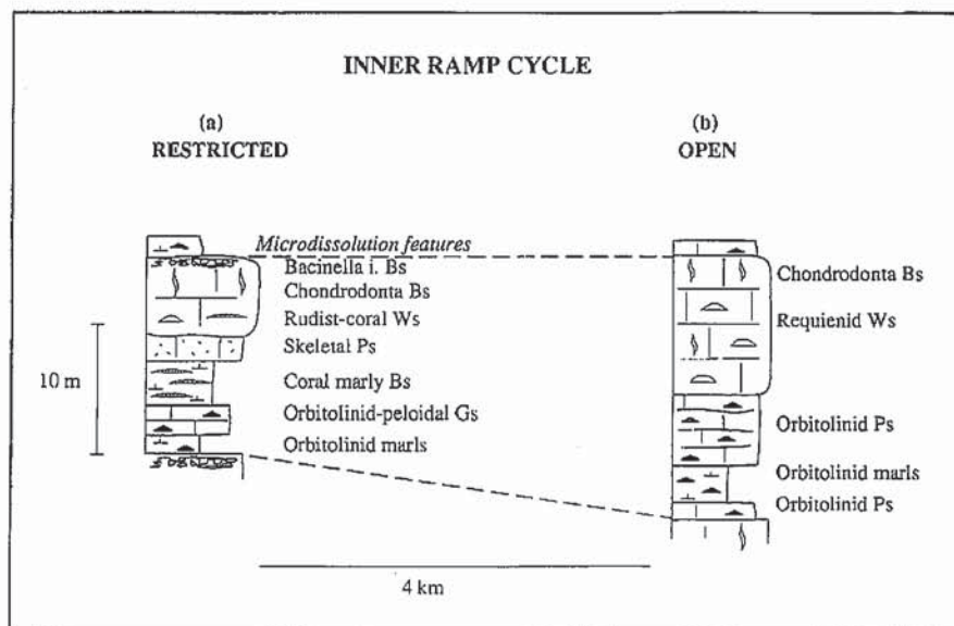
Fig. 3.- Inner carbonate ramp cycles. a) Ideal cycle for the innermost ramp. b) Ideal cycle for the outer settings of the inner ramp.
