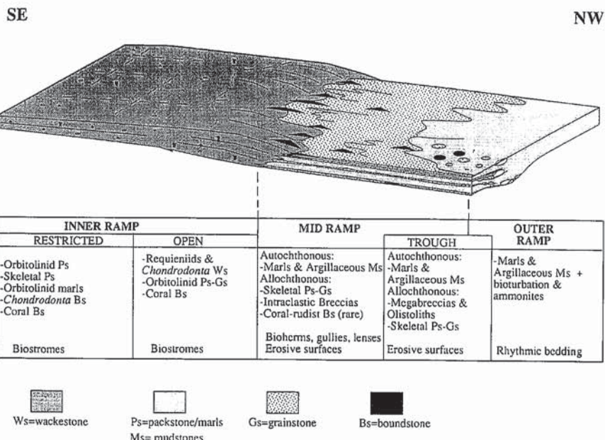
Fig. 2.- Depositional environments and facies distribution for the early Albian Egalezaburu carbonate ramp.
