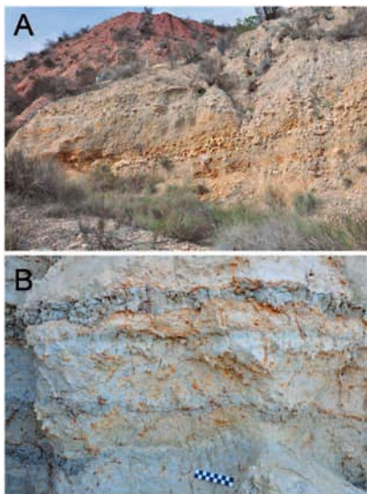
Fig. 4.- A) Gravels and coarse sand. B) Blue lutites and fine sands. See color figure in the web.
