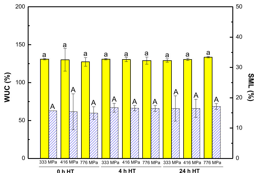
Fig. 8. Water uptake capacity (WUC) and soluble matter loss (SML) of the tablets processed at different compaction pressures and heat-treatment times (HT).
