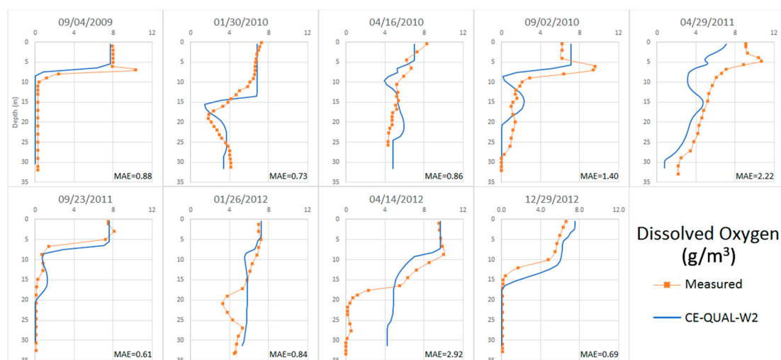
Figure 9. Dissolved oxygen (DO) distribution profiles for different dates in the dry and rainy seasons from a profile near the dam of the Olivargas Reservoir.
