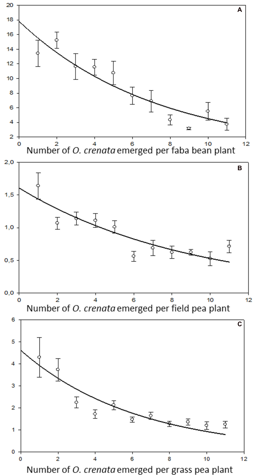
FIGURE 5 | Relationship between average dry weight of individual O. crenata plant and infection severity measured as O. crenata emergence per host plant. (A) Faba bean ( y = 17.82 e^{(-0.14x)} , r^2 = 0.89 , P < 0.0001 ), (B) field pea ( y = 1.61 e^{(-0.11x)} , r^2 = 0.80 , P = 0.0002 ), (C) grass pea ( y = 4.62 e^{(-0.16x)} , r^2 = 0.85 , P < 0.0001 ).
