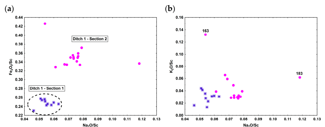
Figure 5. Graphical representation of Fe (a) and K (b) concentration vs. Na concentration (normalized to Sc) in ceramic samples from Ditch 1 of the Santa Vitória enclosure (Portugal).
