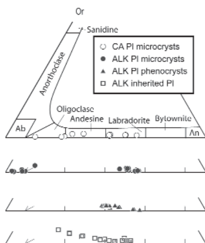
Fig. 2.- Composition (An-Ab-Or) of Pl crystals in the two dike groups.
