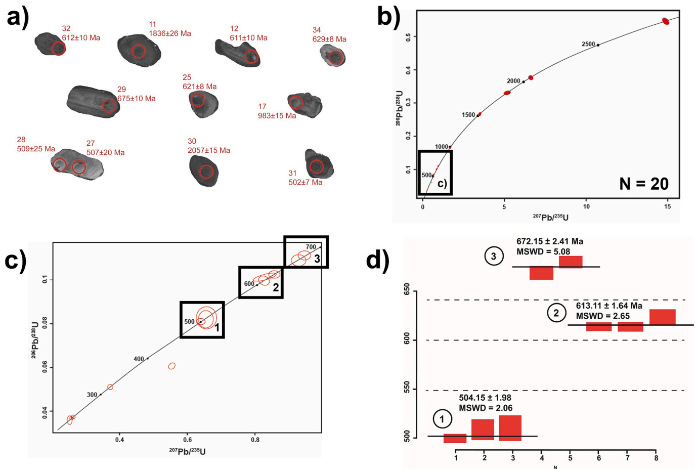
Fig. 9 – U–Pb geochronological results of meta-felsic sample PMT-17: a) Scanning electron microscope (SEM) cathodoluminescence (CL) images of representative zircon grains; b) Wetherill Concordia diagram showing the entire set of LA-ICP-MS analyses; c) Wetherill Concordia diagram between 300 and 700 Ma; and d) ^{238}\text{U}/^{206}\text{Pb} ages weighted mean average diagram for analyses between 500 and 700 Ma.
