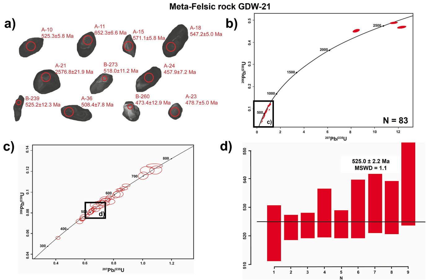
Fig. 8 – U-Pb. geochronological results of meta-felsic sample GDW-21: a) Scanning electron microscope (SEM) cathodoluminescence (CL) images of representative zircon grains; b) Wetherill Concordia diagram showing the entire set of LA-ICP-MS analyses; c) Wetherill Concordia diagram between 300 and 800 Ma; and d) ^{238}\text{U}/^{206}\text{Pb} ages weighted mean average diagram for analyses between 517 and 540 Ma.
