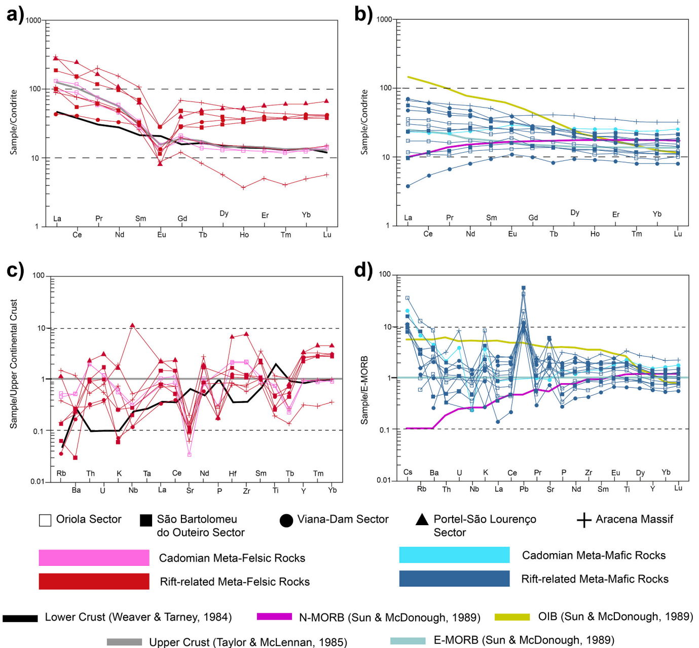
Fig. 4. – a) Chondrite-normalized (McDonough and Sun, 1995) REE patterns for the meta-felsic rock samples; b) Chondrite-normalized (McDonough and Sun, 1995) REE patterns for the meta-mafic rock samples; c) Multi-elemental diagram for the meta-felsic rock samples, normalized to the upper continental crust (Taylor and McLennan, 1995); d) Multi-elemental diagram for the meta-mafic samples, normalized to E-MORB (McDonough and Sun, 1995).
