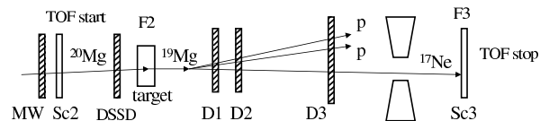
FIG. 1: Sketch of the experimental set-up. The ^{20}\text{Mg} secondary beam was tracked by a silicon strip detector, DSSD, and a multiwire chamber, MW. ^{19}\text{Mg} nuclei were formed in the reaction (^{20}\text{Mg},^{19}\text{Mg})X and products of the decays ^{19}\text{Mg} \rightarrow ^{17}\text{Ne}+p+p were tracked by three planes of silicon micro-strip detectors (D1–D3). ^{17}\text{Ne} ions were identified at foci F2 and F3 as described in the text.
