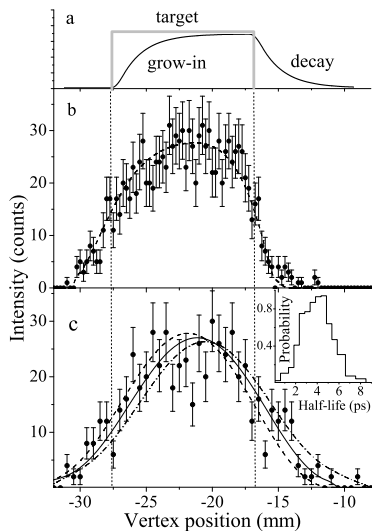
FIG. 3: Profiles of the reaction vertices along the beam direction with respect to the closest micro-strip detector. a) Ideal profiles of prompt (grey curve) and delayed (black curve) decays expected in a thick target. b) Vertex distribution of ^{17}\text{Ne}+p+p events gated by large p-^{17}\text{Ne} angles (and thus large p-^{17}\text{Ne} relative energies), which corresponds to short-lived excited states in ^{19}\text{Mg} (full circles with statistical uncertainties). The dashed curve shows the Monte Carlo simulations of the detector response for the 2p-decay ^{19}\text{Mg}^* \rightarrow ^{17}\text{Ne}+p+p with T_{1/2}=0 . c) The same as b) but gated by small p-^{17}\text{Ne} angles corresponding to the “ground state” group in Fig. 2b. The dashed curve depicts a simulation of the 2p-decay component with T_{1/2}=0 . The solid and dash-dotted curves are fits to the data assuming a mixture of 25% of the T_{1/2}=0 component and 75% of the radioactivity component with T_{1/2} values of 4 and 8 ps, respectively. The insert shows the probability (as a function of the assumed half-lives) that the simulations match the data.
