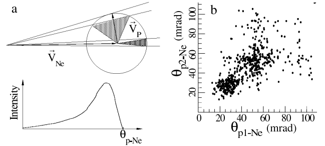
FIG. 2: a) Illustration of the kinematical enhancement of angular correlations of decay products at the maximum possible angles between the decay products. b) Angular p- 17 Ne correlations obtained from the measured 17 Ne+p+p events by selecting their vertex position inside the target (full circles).
