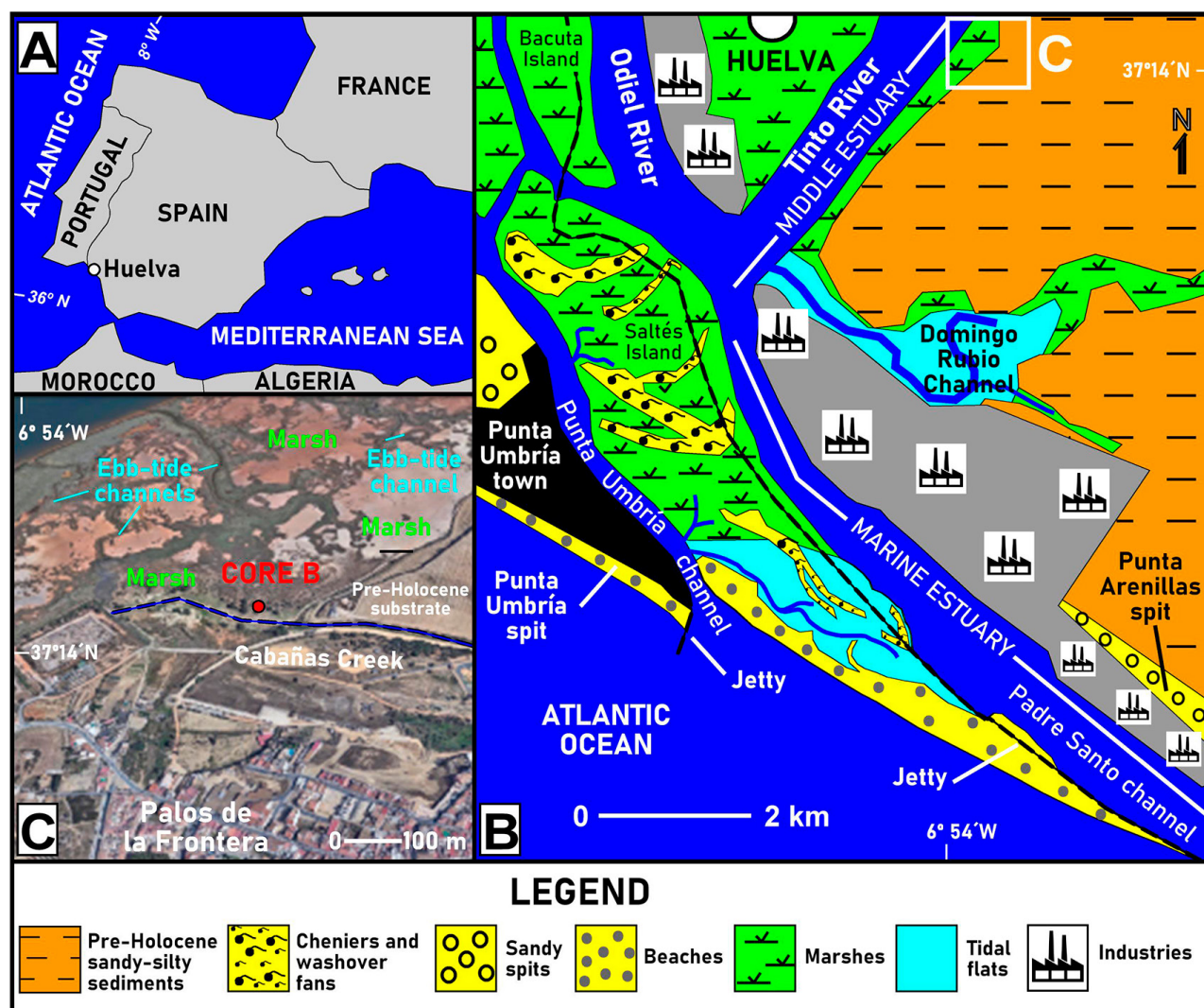
Fig. 1. – A-B, location and geomorphological map of the Tinto River estuary; C, location of core B.
