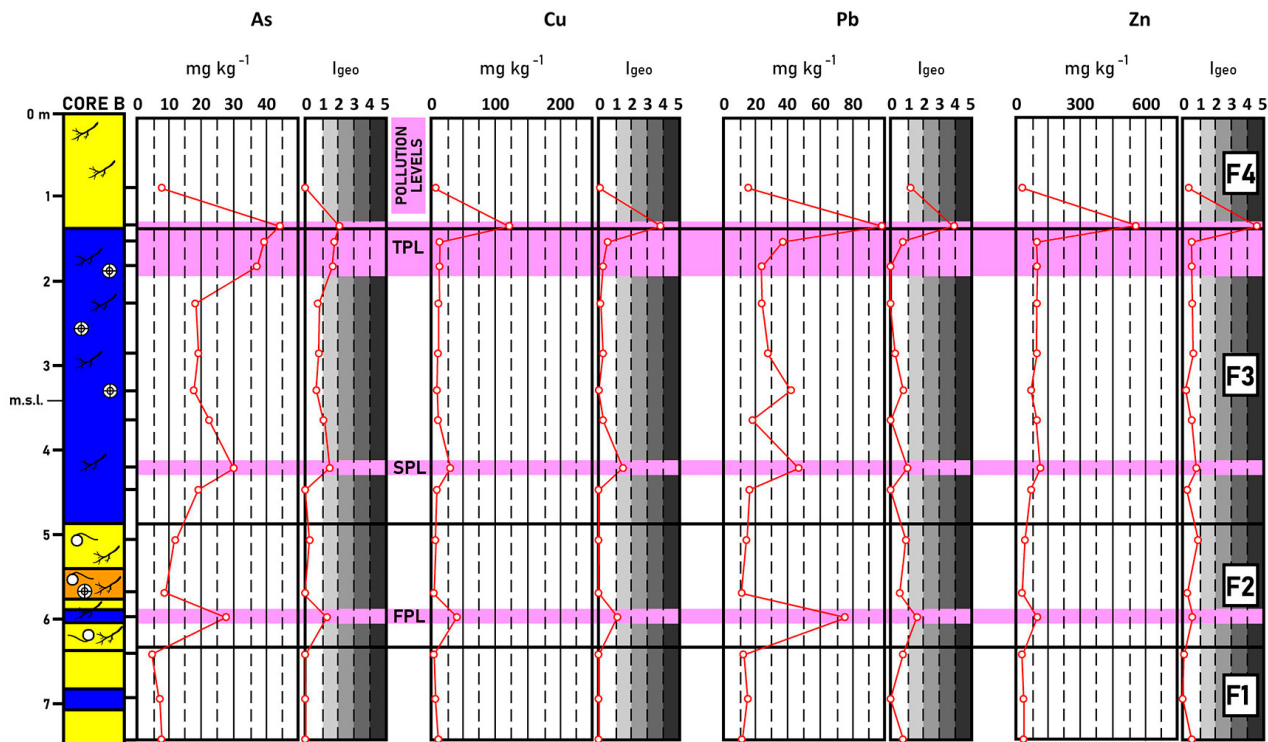
Fig. 3. – Geochemistry of core B (in mg kg -1 ). FPL: first pollution level; SPL: second pollution level; TPL: third pollution level.
