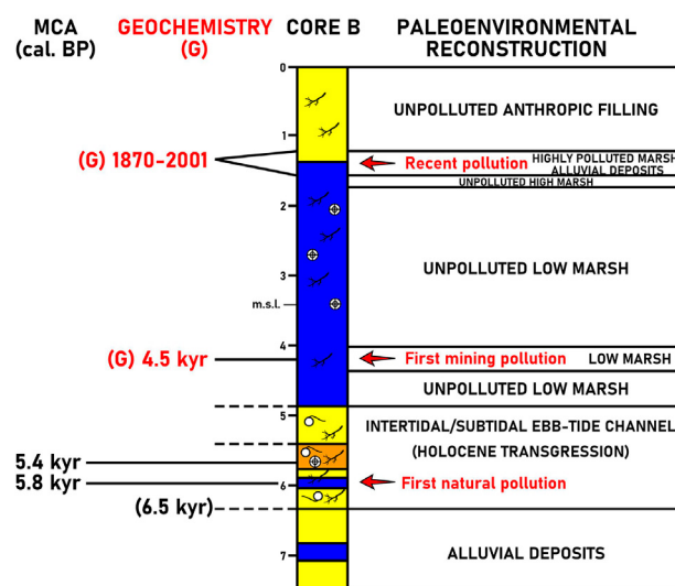
Fig. 6. – Paleoenvironmental evolution of core B. MCA: mean calibrated age.
