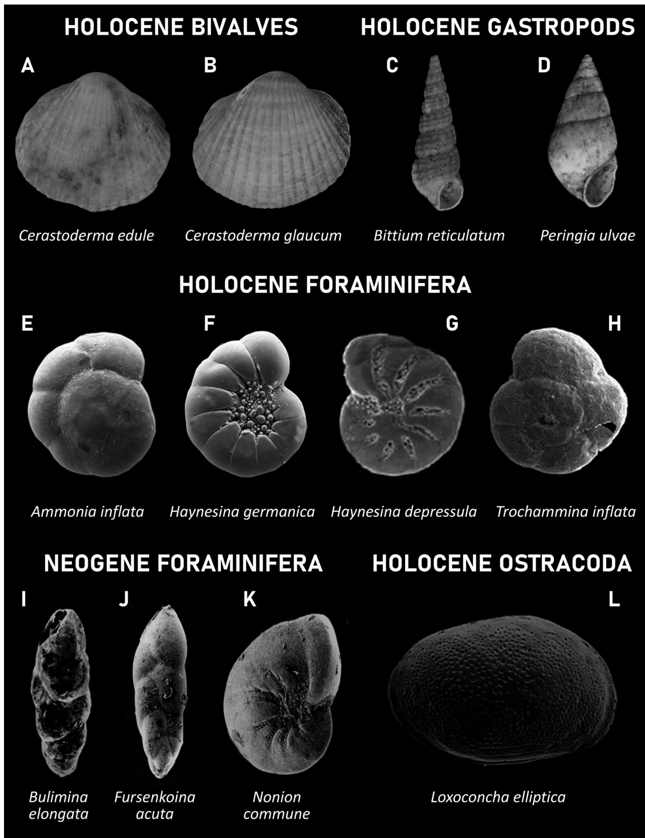
Fig. 5. – Main species of core B. Scale not respected.
