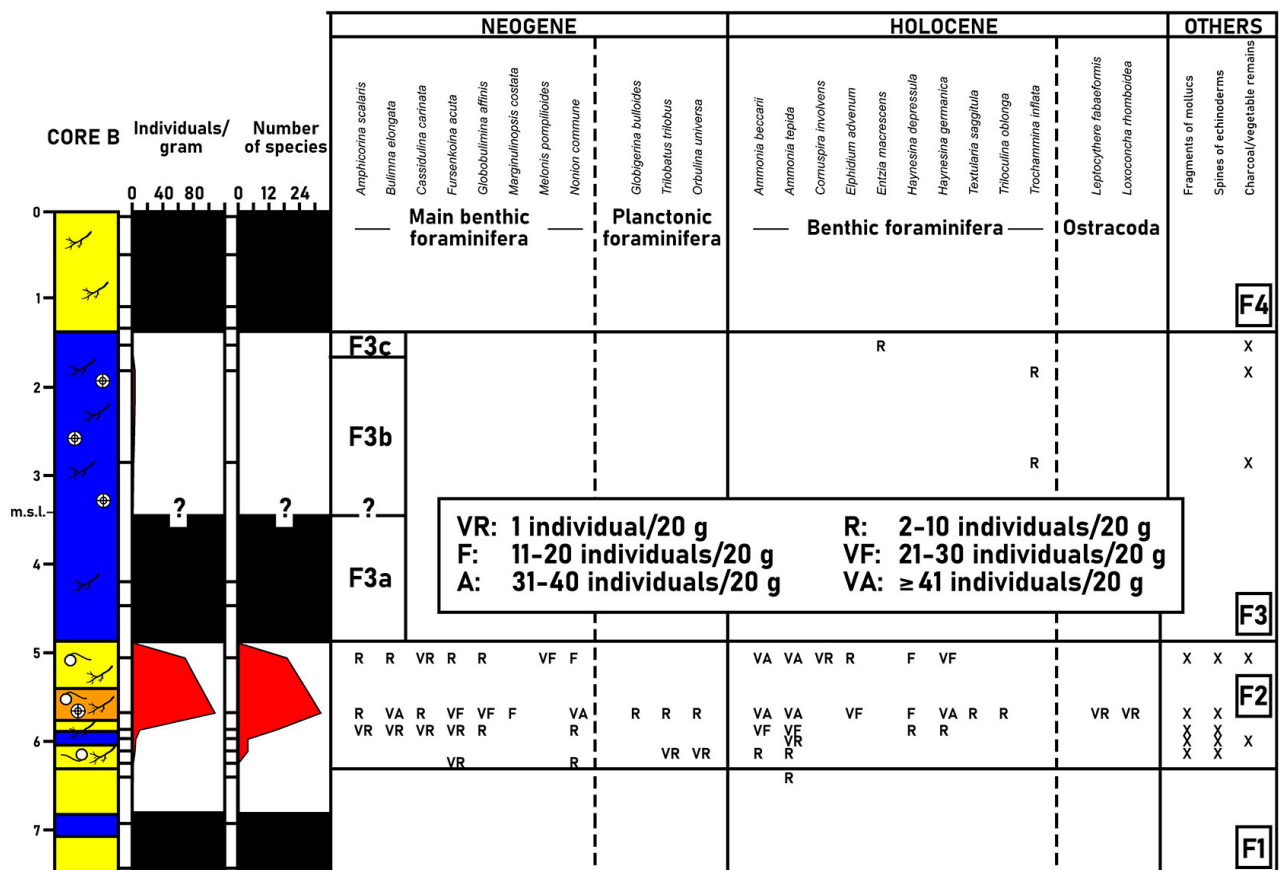
Fig. 4. – Palaeontological record of core B.
