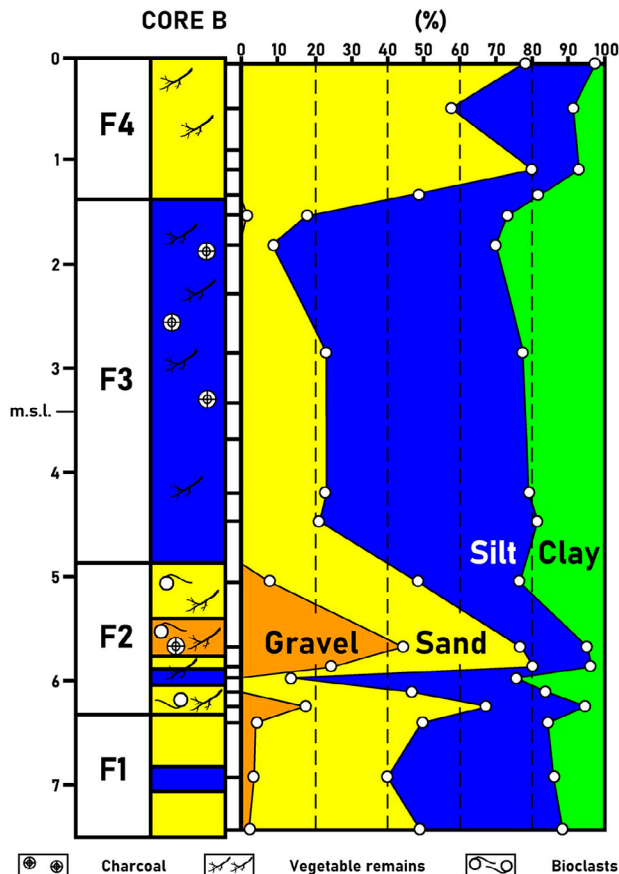
Fig. 2. – Textural analysis of core B.
