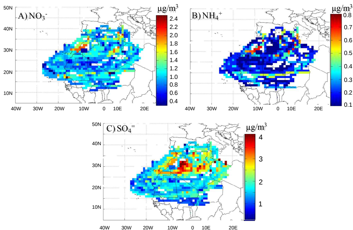
Fig. 10. Median concentrations at receptor (MCAR) plots for nitrate, ammonium and sulphate concentrations in the \text{PM}_{10} fraction.
