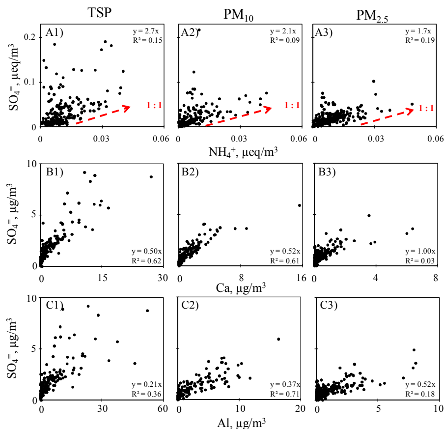
Fig. 4. Concentrations of sulphate versus ammonium, calcium and aluminium.
