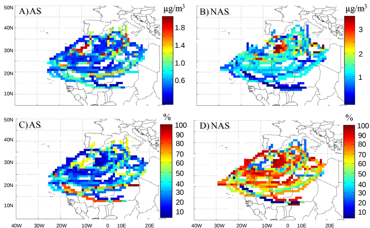
Fig. 14. Median concentrations at receptor (MCAR) plots for ammonium sulphate (AS) and non-ammonium sulphate (NAS), in the \text{PM}_{10} fraction, in terms of absolute concentration (A–B) and contribution to total sulphate (C–D).
