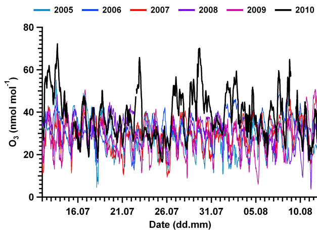
Fig. 2b. Ozone (30 min average) recorded in Hyytiälä between July and August from 2005–2009 from mast at 16.8 m and 2010 from 33.6 m.
