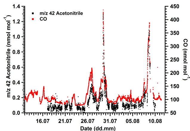
Fig. 7. Acetonitrile ( \text{CH}_3\text{CN} ) and Carbon monoxide (CO) mixing ratios (5 min averages) for the duration of HUMPPA-COPEC campaign measured at the HUMPPA tower.
