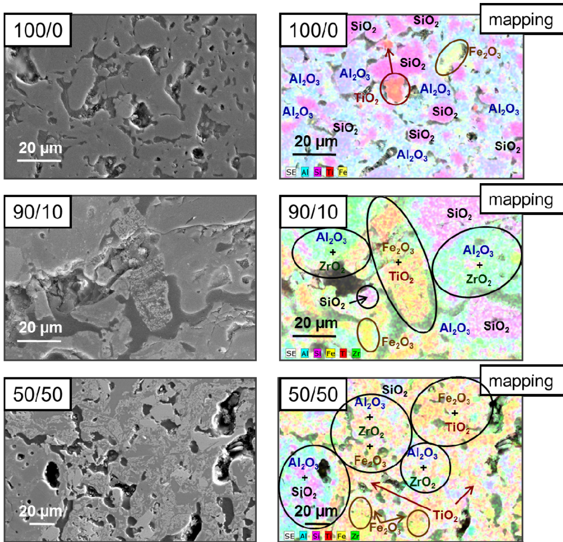
Figure 9. FESEM images and elemental mappings on polished surfaces of fired 100/0, 50/50 and 90/10 samples.
