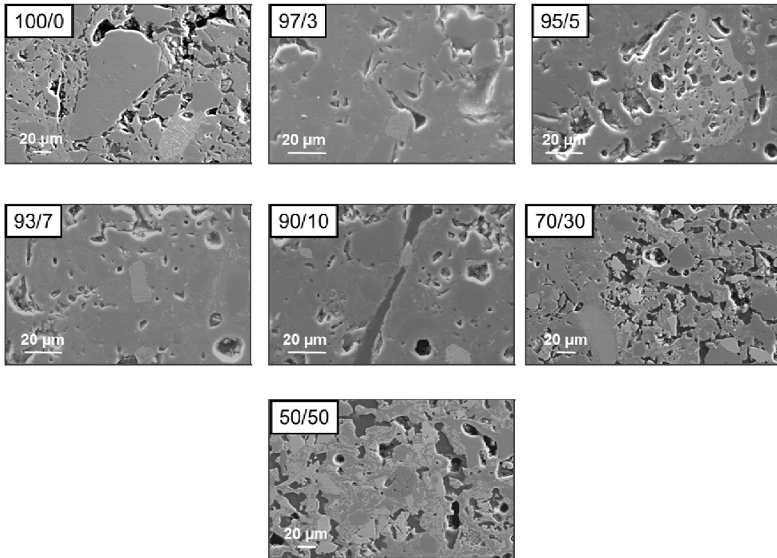
Figure 8. Secondary electron images (high magnification) on polished surfaces of fired tiles
