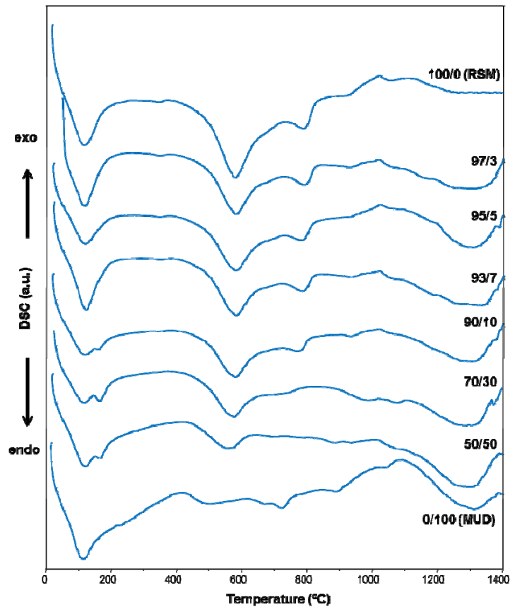
Figure 6. DSC curves (25-1450°C, 50°C/min); a) 97/3, b) 95/5, c) 93/7, d) 90/10, e) 70/30 and f) 50/50.
