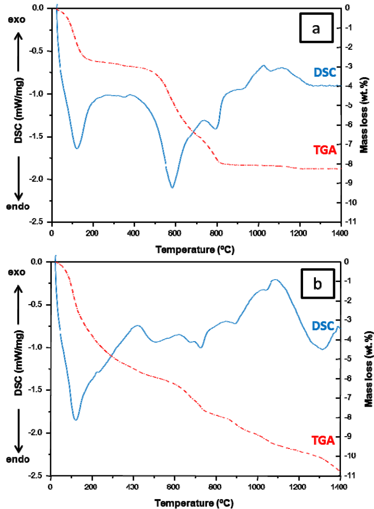
Figure 4. DSC/TG curves (25-1450°C, 50°C/min); a) RSM and b) tionite.
