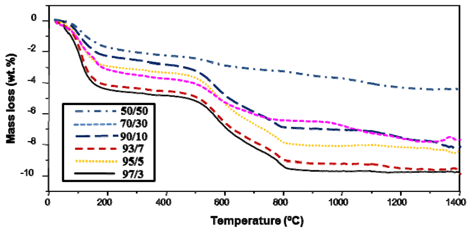
Figure 5. TG curves (25-1450°C, 50°C/min) of 97/3, 95/5, 93/7, 90/10, 70/30 and 50/50.
