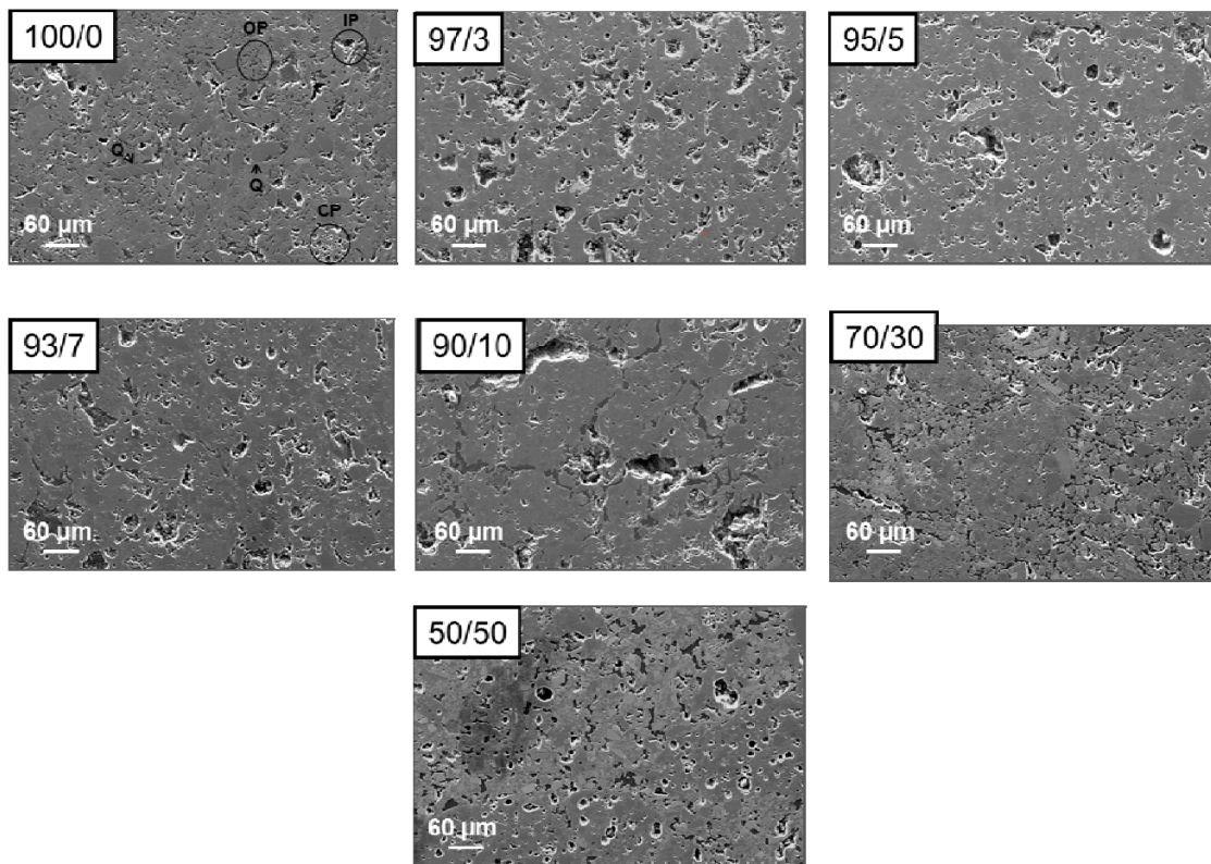
Figure 7. Secondary electron images (low magnification) on polished surfaces of fired tiles . Q: quartz; OP: open porosity; CP: close porosity and IP: interparticle porosity.
