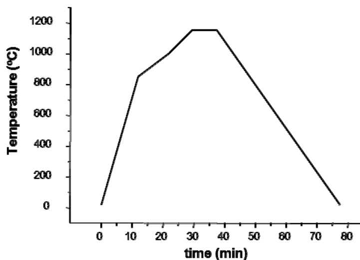
Figure 1. Heating cycle used for the fast-firing of ceramic tiles
