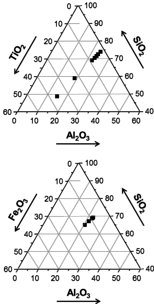
Figure 3. Location of tested composition in the SiO 2 -Al 2 O 3 -TiO 2 and SiO 2 -Al 2 O 3 -Fe 2 O 3 ternary systems
