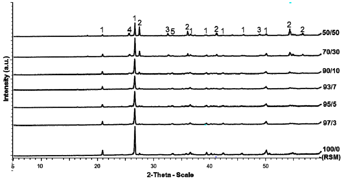
Figure 2. XRD patterns of fired tiles. [1]: Quartz ( \text{SiO}_2 ); [2]: Rutile ( \text{TiO}_2 ); [3]:
