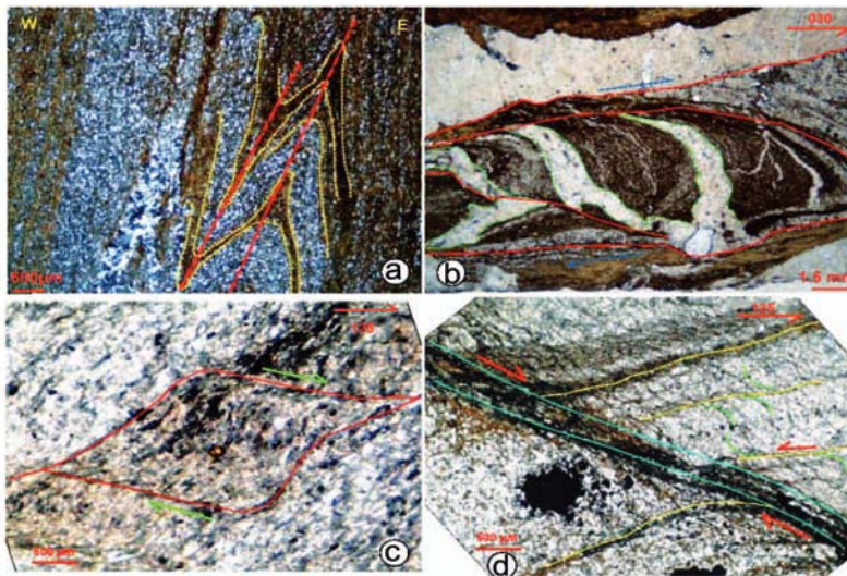
Fig. 4- Microscope photographs of some structural features. a) Sample 017-1: microfold affecting S0/S1, thickening in the fold hinge; b) sample 008-2: dextral shear zone with crown milky quartz; c) sample 32-2: shallowly dipping shear zones cross cutting the bedding; d) sample 34A-2: tourmaline vein (marked with cyan lines) affected by a shallowly dipping dextral shear zone with tin mineralization with S0/1 with yellow colour, S2 in blue colour. See color figure in the web.
