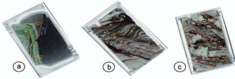
Fig. 3- Thin sections showing the structural features in BLJ. a) sample 017-1: microfold affecting S0/S1, S2 crenulation cleavage and a reverse fault that shows the fold-and-thrust structure. b) Sample 34-A: shallowly dipping C-S structure with dextral sense. c) Sample 32: brittle-ductile, shallowly dipping structure. See color figure in the web.
