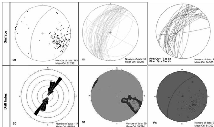
Fig. 5.- Stereoplots of structural features (S0 stratification, S1 schistosity and veins) obtained from the surface (top row) and from the drilling core (bottom row). See color figure in the web.
