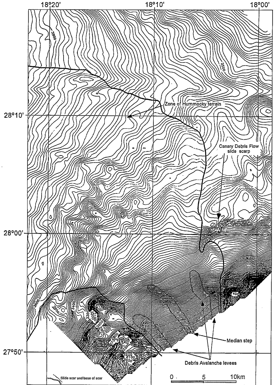
Fig. 3.- Detailed bathymetry of the El Golfo debris avalanche headwalls. A zone of hummocky terrain appears at the foot of these scarps. This zone also truncates a scarp roughly oriented NE which could correspond to one of the source areas of the former Canary debris flow. Situation in Fig. 2.
