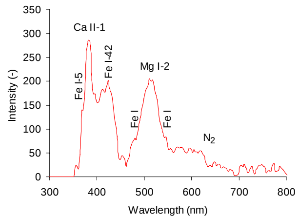
Figure 5. Emission spectrum of the SPMN210712 bolide.
