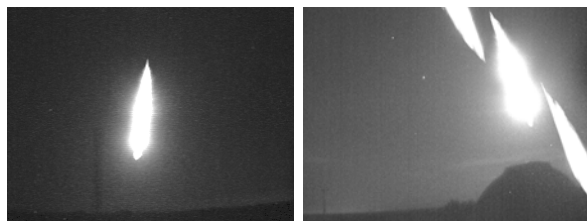
Figure 1. Composite image of the fireball as imaged from El Arenosillo (left) and La Hita (right).
