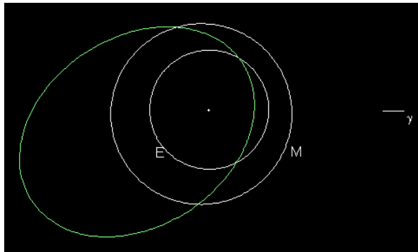
Figure 3. Projection on the ecliptic plane of the orbit of the parent meteoroid.
