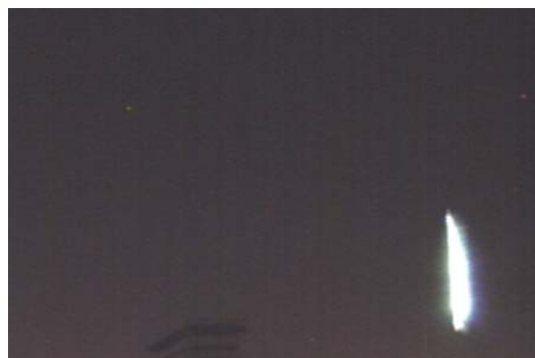
Figure 2. Composite image taken by a low-sensitivity colour CCD camera operating from Sevilla.
