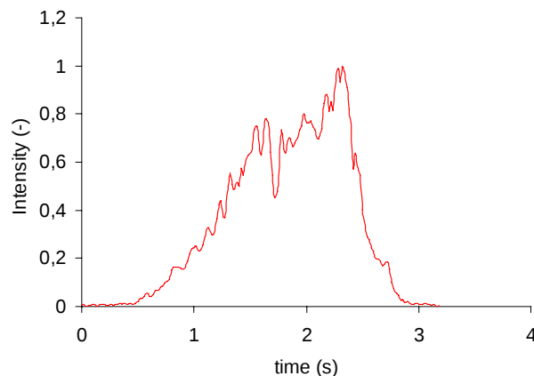
Figure 4. Light curve (relative pixel intensity vs. time) of the SPMN210712 fireball.
