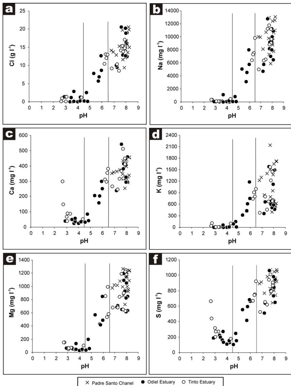
Fig. 2.- Bivariant plots of well-correlated \text{Cl}^- , \text{Na}^+ , \text{Ca}^{2+} , \text{K}^+ , \text{Mg}^{2+} and \text{SO}_4^{2-} vs. pH of the dissolved phase of estuarine water samples.
