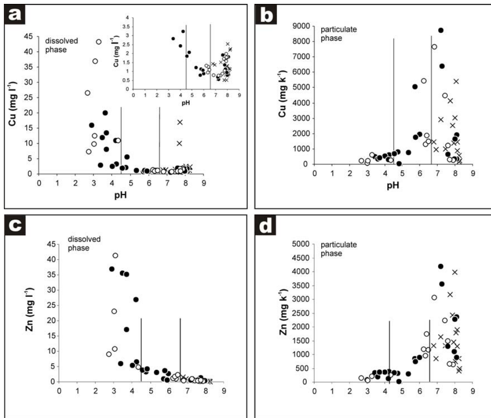
Fig. 3.- Relationships pH vs. \text{Zn}^{2+} and \text{Cu}^{2+} concentration in water samples: (a) dissolved \text{Cu}^{2+} vs. pH (b) particulate \text{Cu}^{2+} vs. pH (c) dissolved \text{Zn}^{2+} vs. pH and (d) particulate \text{Zn}^{2+} vs. pH.
