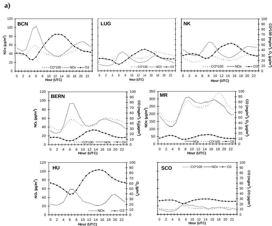
Fig. 2. Daily cycle of: (a) Gaseous pollutants concentrations (CO, NO x and O 3 ), (b) Black carbon (BC) and Number concentration (N), (c) BC and PM 10 , and (d) N and SO 2 levels for each monitoring site.
