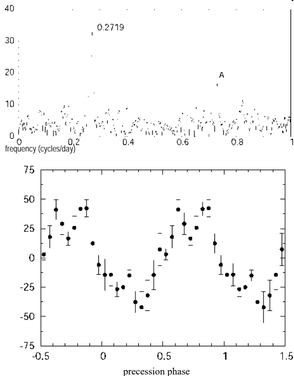
Figure 9. Upper frame : power spectrum of the departures of eclipse timings from the ephemeris given in Eq. (1). A significant peak occurs at 0.2719(10) \text{c d}^{-1} , the same (nodal) frequency, N , characterizing the large variations in light seen in Fig. 2. The peak labelled with 'A' is an alias centred at frequency 1 - N . Lower frame : fold of these residuals on the nodal frequency according to the ephemeris given in Eq. (2), showing a periodic effect with a semi-amplitude of 33.3(9) s.
