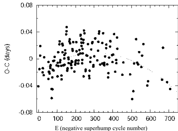
Figure 10. O - C diagram of the 0.1867 d superhump maxima with respect to the test ephemeris given in Eq. (3).
