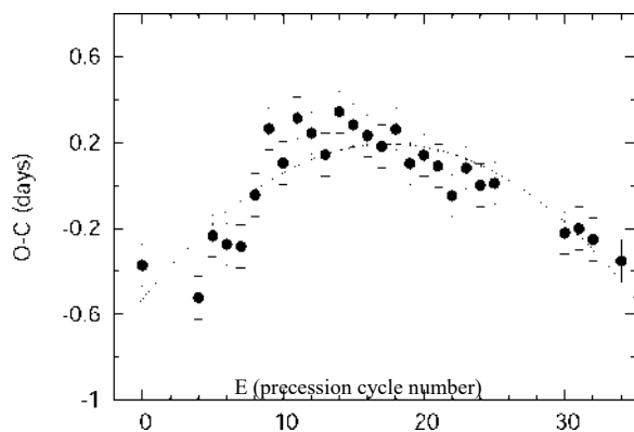
Figure 6. O - C residuals of the timings of maximum light (Table 4) on the 3.68 day cycle as determined from the ephemeris given in Eq. (2). The dashed curve represents the best quadratic fit, from which we infer that the nodal period changes by \sim 0.2 d over the 5-month campaign.
