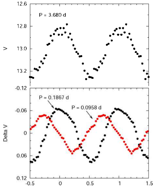
Figure 5. Upper frame : mean light curve folded on the nodal ( N ) frequency (0.2717 \text{c d}^{-1} or 3.68 d) relative to the ephemeris given in Eq. (2). Lower frame : mean light curve after removing the nodal and orbital signals folded on the f_{\text{orb}} + N frequency (5.3562 \text{c d}^{-1} or 0.1867 d, black points) and the 2f_{\text{orb}} + N frequency (10.4391 \text{c d}^{-1} or 0.0958 d, red points) relative to the ephemeris given in Eq. (3).
