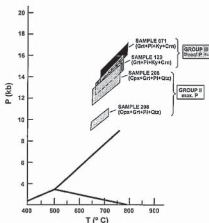
Fig. 1.- P-T diagram showing thermobarometric data for the mineral assemblages of coronas of groups II and III. Stability of the \text{Al}_2\text{SiO}_5 polymorphs according to Holdaway (1971).
