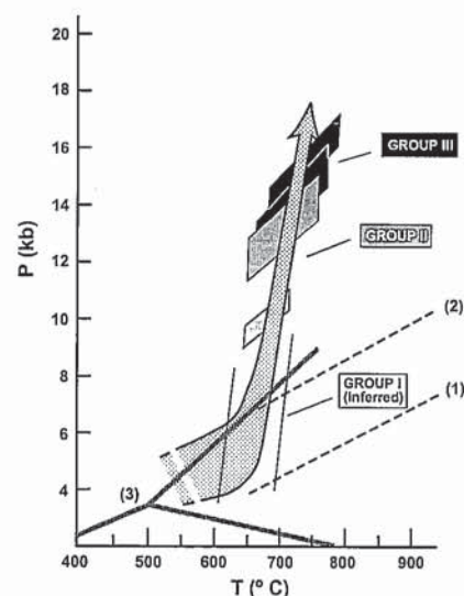
Fig. 2.- P-T path suggested for the coronitic metagabbros of the Sobrado Unit. P-T conditions for the development of group I, II and III coronas are also shown, together with lower (1) and upper (2) conditions for the beginning of garnet stability in mafic granulites (after Ringwood and Green, 1966 and Green and Ringwood, 1967). Stability of the \text{Al}_2\text{SiO}_5 polymorphs (3) after (Holdaway, 1971).
