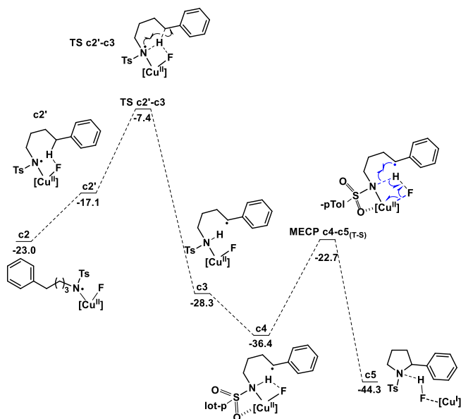
Scheme 6. Free energy profile of the C-H activation and cyclization steps of reaction with 1k as the substrate. Energies in kcal/mol. ([Cu] = Tp + Cu).
