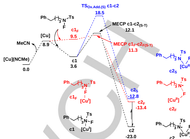
Scheme 5. Free energy profile of the N–F activation step of reaction with 1k as the substrate. Energies in kcal/mol. ([Cu] = Tp x Cu).
