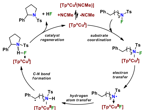
Scheme 7. Mechanistic proposal based on combined experimental and computational data.
