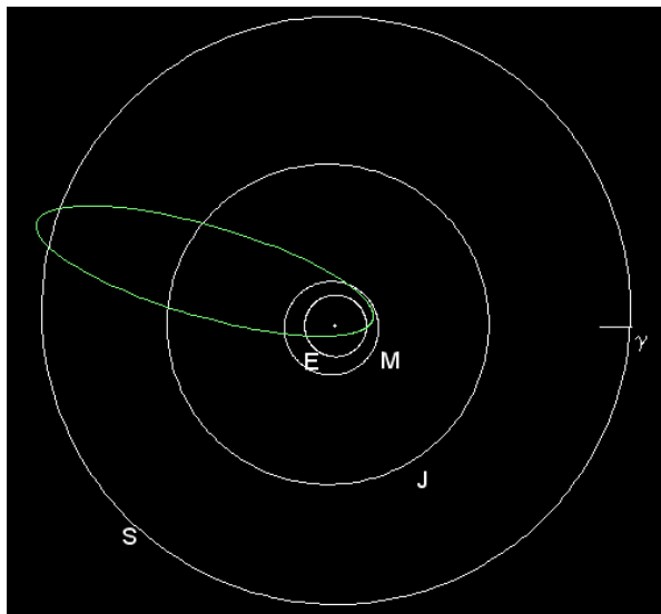
Figure 3. Orbit of the parent meteoroid projected on the ecliptic plane.
