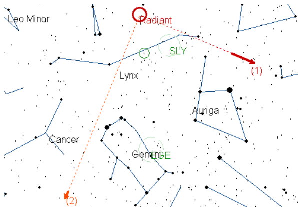
Figure 2. Apparent path of the superbolide as recorded from Sierra Nevada (1) and Sevilla (2).
