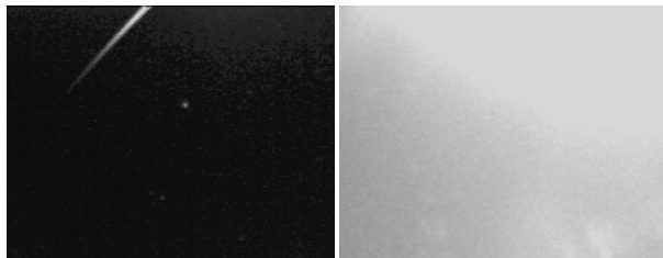
Figure 1. Composite image of the fireball, taken from Sierra Nevada, during its beginning (left) and maximum phase (right).
