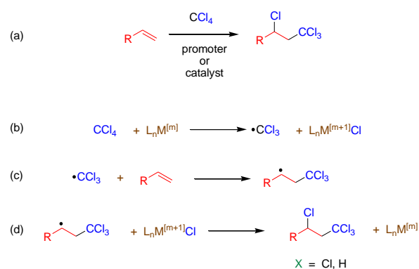
Scheme 1. (a) The Kharasch reaction. (b-d) Commonly proposed mechanism for the metal-mediated Atom Transfer Radical Addition (ATRA) reaction
