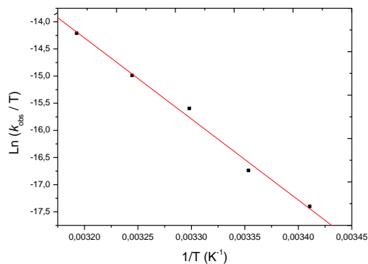
Figure 7. Eyring plot for the ATRA reaction of styrene and \text{CCl}_4 catalyzed by 1 . Conditions [\mathbf{1}]:[\text{styrene}]:[\text{CCl}_4] = 1:300:1200 ; [cat] = 1.5 mM; solvent, benzene- d_6 .
