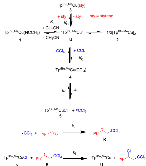
Scheme 6. The different steps in the ATRA reaction of styrene and \text{CCl}_4 using complex 1 as the catalyst precursor
