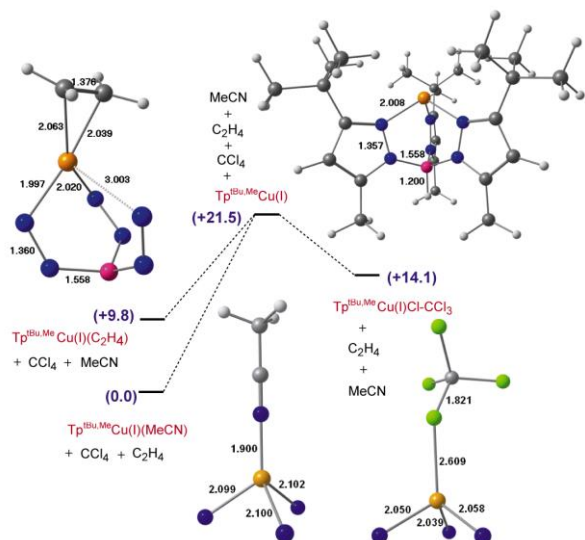
Figure 8. Potential energy diagram for the equilibria connecting the initial form of the catalyst with the reaction channel (energy values are in kcal mol -1 and spin densities at selected atoms are shown in italics).
