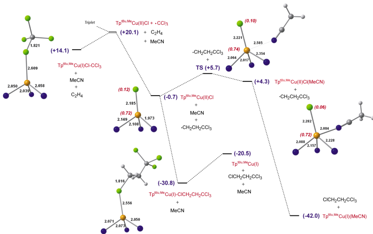
Figure 9. Potential energy diagram for the ATRA of CCl 4 to C 2 H 4 by \text{Tp}^{\text{tBu,Me}}\text{Cu}(\text{I}) complex. (energy values are in kcal mol -1 and spin densities at selected atoms are shown in italics).
