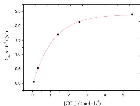
Figure 6. Dependence of k_{\text{obs}} with the \text{CCl}_4 concentration for the ATRA reaction of styrene and \text{CCl}_4 catalyzed by 1 . Conditions: [cat] = 4.6 mM; solvent, benzene- d_6 .
