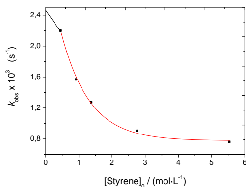
Figure 5. Dependence of k_{\text{obs}} for product formation with the olefin concentration for the ATRA reaction of styrene and \text{CCl}_4 catalyzed by 1 . Conditions: [cat] = 4.6 mM; solvent, benzene- d_6 .
