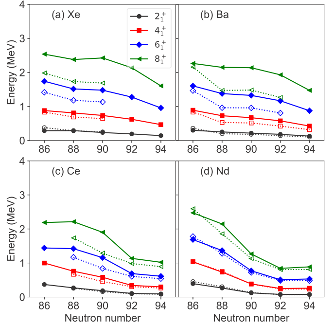
FIG. 4. The low-energy excitation spectra of positive-parity even-spin yrast states in ^{140-148}\text{Xe} , ^{142-150}\text{Ba} , ^{144-152}\text{Ce} and ^{146-154}\text{Nd} , computed by diagonalizing the mapped sdf -IBM Hamiltonian (1), are shown as functions of the neutron number. Experimental data have been taken from Ref. [76].
