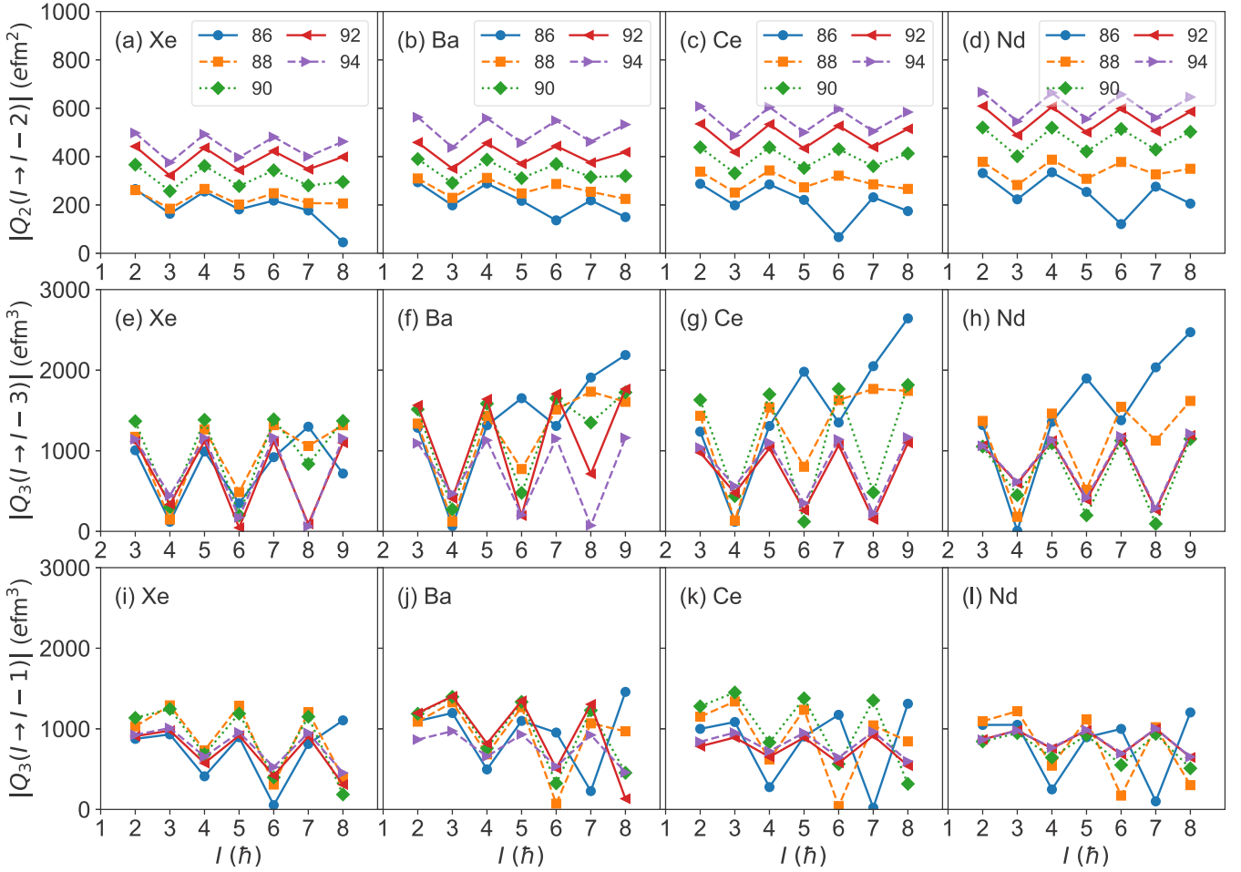
FIG. 12. The theoretical quadrupole Q_2(I \rightarrow I-2) (top), octupole Q_3(I \rightarrow I-3) (middle), and Q_3(I \rightarrow I-1) (bottom) moments in \text{efm}^k units are plotted as functions of the spin I . Even- (Odd-) I values correspond to positive- (negative-) parity states.
