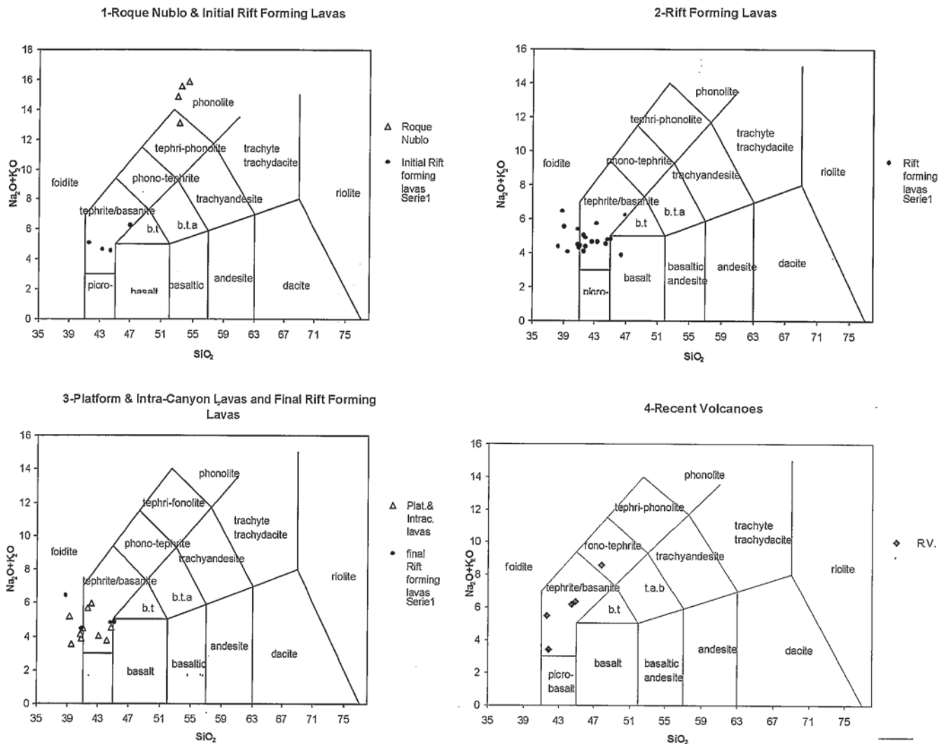
Fig. 2.- TAS classification of studied rocks arranged form older to recent ones (2.1 to 2.4, see text for explanation)
