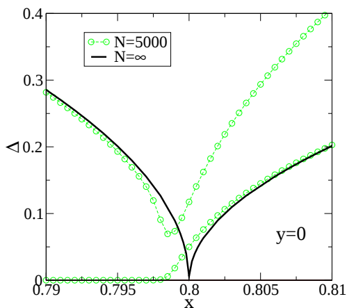
FIG. 6: (Color online) Same as Fig. 5 but for y = 0 . The full line is the analytical result for the gap, while the open dots correspond to the first two excited states for N = 5000 .
