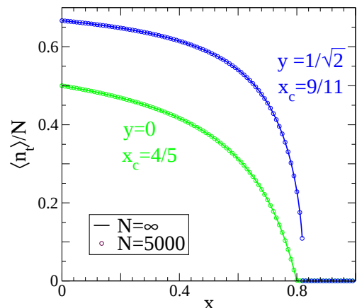
FIG. 4: (Color online) Variation of the order parameter as a function of x near the critical point. Full line are the analytical results for N = \infty and circles are numerical results for N = 5000 . The jump is clearly observed for y \neq 0 .
