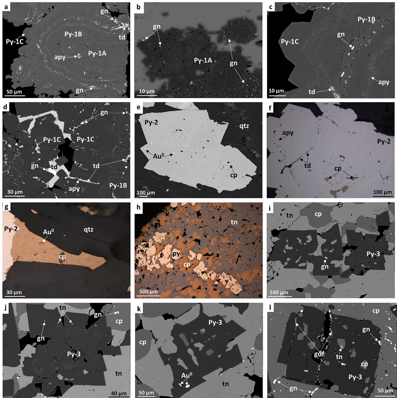
Fig. 2. Reflected light and BSE images of different pyrite types from polymetallic (Masa Verde) and Cu-rich (La Magdalena) of the IPB. (a) Py-1 consists of framboids relicts (Py-1A) in the cores surrounded by concentric colloform bands (Py-1B) ended by faceted outlines (Py-1C). Note that Py-1 includes subhedral arsenopyrite (apy) sealing open spaces in Py-1A but galena (gn) and tetrahedrite (td) occur within Py-1B concentric layers. (b) Fine galena micron-sized inclusions in the framboidal pyrite of Py-1A. (c) Micron-sized inclusions of galena and arsenopyrite oriented parallel to colloform pyrite concentric layers and tetrahedrite lining interstices between Py-1B bands. (d) galena, tetrahedrite and arsenopyrite lining open spaces in the outer faceted rims of Py-1C. (e, f) Euhedral pyrite with spongy cores (Py-2). Note that chalcopyrite (cp) and tetrahedrite inclusions are mainly filling interstices in spongy cores whereas inclusions of arsenopyrite and native gold (Au) are mainly concentrated towards outer rims. (g) native gold particle included in chalcopyrite intergrown with Py-2. (h, i) Euhedral pyrite (Py-3) included in a matrix formed by an intergrowth of chalcopyrite and tennantite (tn). (j) Detail of the euhedral pyrite showing As-rich zoned cores and, galena and tennantite inclusions. (k) Tennantite, chalcopyrite and native gold replacing euhedral pyrite. (l) Gersdorffite (gdf) lining late fractures in Py-3 Tennantite, chalcopyrite and galena are also observed replacing Py-3.
