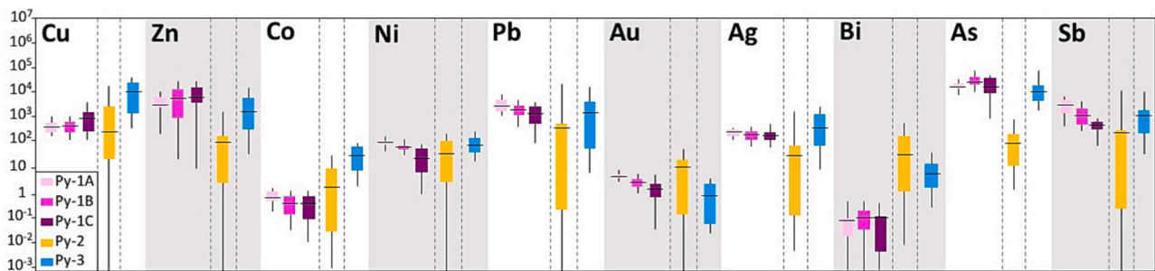
Fig. 7. Concentration of minor and trace elements in different textural pyrite types represented as box plot. Only inclusion-free LA-ICP MS analysis data were included in this plot ( n = 133 ). Data are plotted ppm on a vertical logarithmic scale, including minimum, median and maximum values for each single element.
