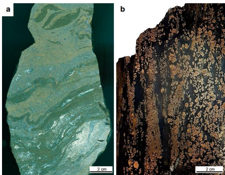
Figure 2. Massive sulfides generated by replacement of: (a) volcaniclastic rocks replaced by polymetallic sulfides, from Aguas Teñidas, showing of dacitic volcanic rocks embedded and corroded by sulfides. The banded facies show an original slumping fold, including very thin bands of sedimentary pyrite bearing shale. Coarse sized bands correspond to porous volcaniclastic beds pervasively replaced by sulfides (i.e., Galena, sphalerite, pyrite and chalcopryrite) and carbonates; and (b) black shales from Cueva de la Mora, where pyrite aggregates pervasively replace the rock.
