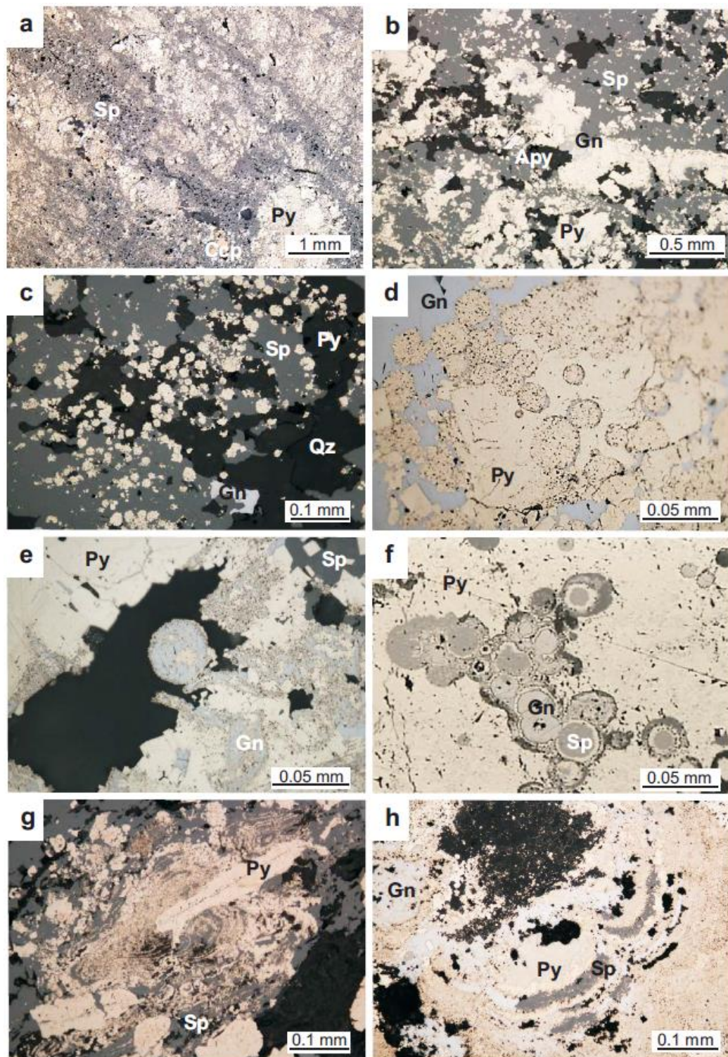
Figure 6. Optical microscope images of polymetallic mineralizations from several massive sulfide deposits of the IPB. (a) pyrite (Py) banded textures partially replaced by sphalerite (Sp) along high porosity bands; (b) advanced replacement textures on banded pyrite by polymetallic sulfide ore; (c) framboidal pyrite relicts partially embedded in sphalerite; (d) framboidal pyrite recrystallized and replaced by galena (Gn); (e) galena pseudomorph generated by replacement of framboidal pyrite; (f) aggregates of framboidal pyrite replaced by a second pyrite generation and late galena and sphalerite filling and replacing framboids and other open spaces; (g) selective replacement of colloform pyrite by sphalerite and galena. Massa Valverde deposit (a), Magdalena deposit (b,c,g,h) and Frailes deposit (d–f).
