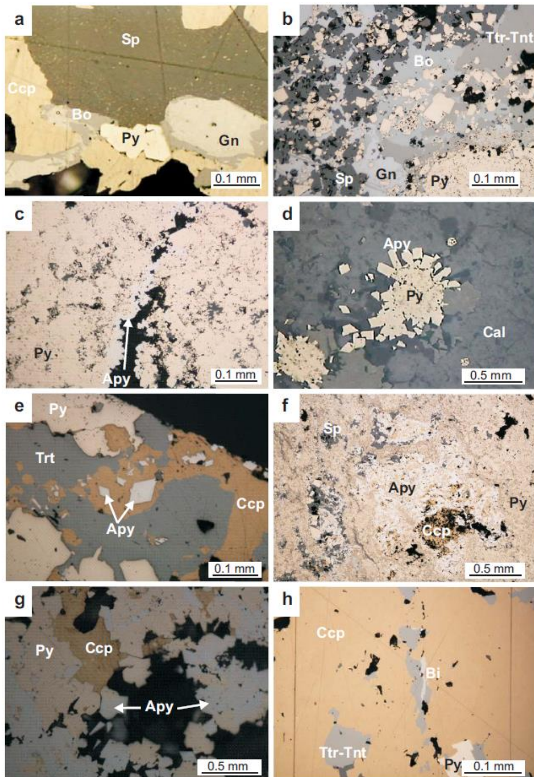
Figure 8. Optical microscope images of polymetallic mineralizations with As–Sb from several massive sulfide deposits of the IPB. (a,b) Late Cu–Pb–As–Sb sulfosalts, including boulangerite (Bo) and tetrahedrite–tennantite (Ttr–Tnt) replacing suitable sulfides; (c) late arsenopyrite (Apy) filling open spaces in pyrite aggregates; (d) fine grained pyrite overgrown by idiomorphic late arsenopyrite; (e) interstitial chalcocopyrite (Ccp) in pyrite (Py) partially replaced by tetrahedrite–tennantite. Idiomorphic arsenopyrite crystals are also present; (f) arsenopyrite replacing pyrite and overgrowing former sulfides; (g) late arsenopyrite filling open space in a pyrite aggregates; (h) veinlet of bismuthine (Bi) associated with tetrahedrite–tennantite in chalcocopyrite ore. Frailes deposit (a,b,d) and Magdalena deposit (c,e,g,h).
