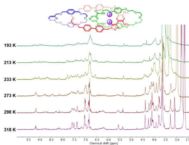
Fig. 4 Variable temperature ^1\text{H} NMR spectra of 1 (acetone- \text{d}_6 , 500 MHz).
