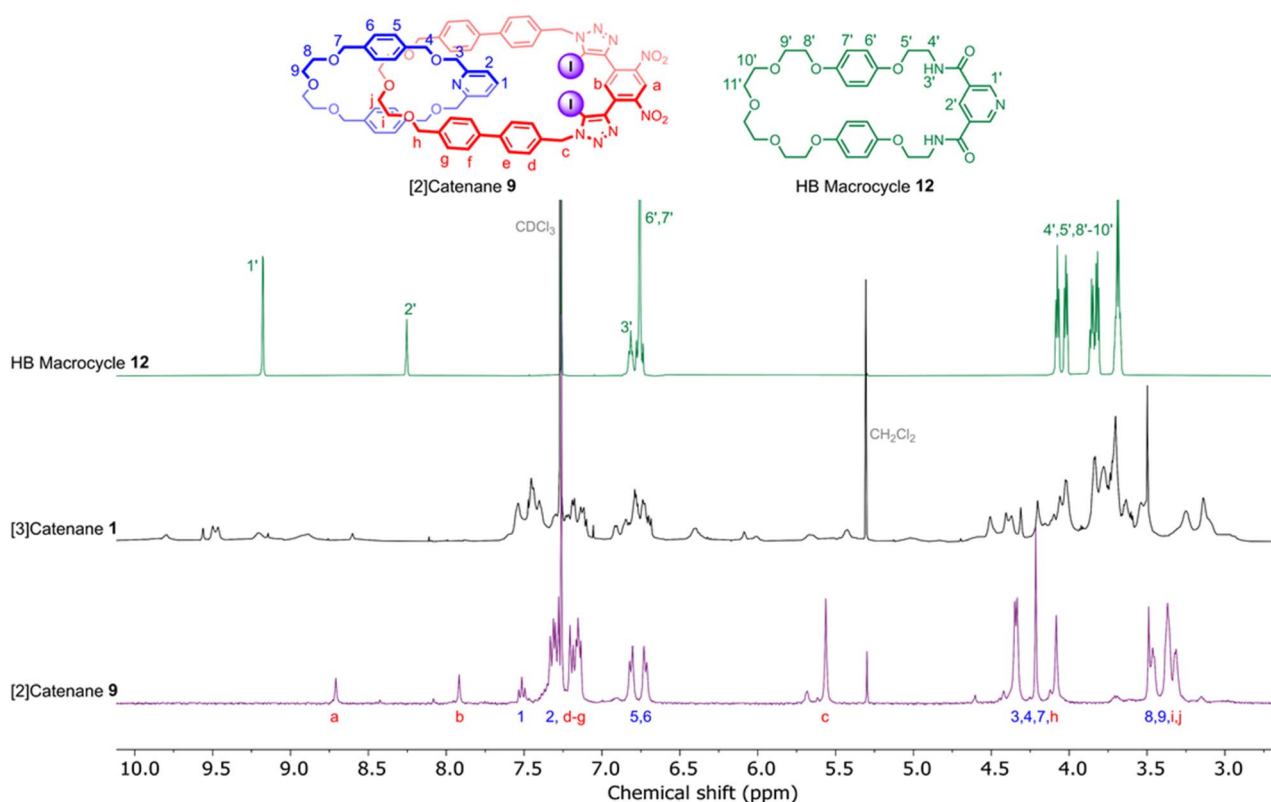
Fig. 3 Stacked ^1\text{H} NMR spectra of HB macrocycle 12 (top), [3]catenane 1 (middle) and [2]catenane 9 (bottom) ( \text{CDCl}_3 , 500 MHz, 298 K).
