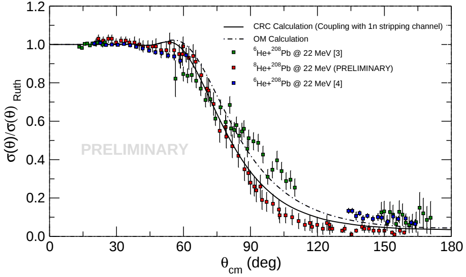
Figure 1. Angular distribution of the elastic cross section, normalized to the corresponding Rutherford cross section, for the systems ^8\text{He}+^{208}\text{Pb} and ^6\text{He}+^{208}\text{Pb} at 22 MeV. See text for details.
