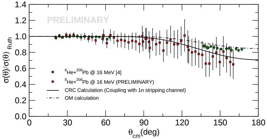
Figure 2. Angular distribution of the elastic cross section, normalized to the corresponding Rutherford cross section, for the systems ^8\text{He}+^{208}\text{Pb} and ^6\text{He}+^{208}\text{Pb} at 16 MeV. See text for details.
