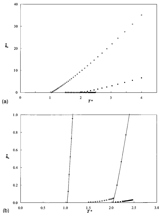
FIG. 5. Global phase diagram in P^* - T^* representation for linear rigid chain molecules of three and five tangent LJ segments as obtained from the simulations of this work. See Fig. 4 for details of the symbols. (b) shows the P^* - T^* projection at low pressures (the lines are guides to the eyes).
