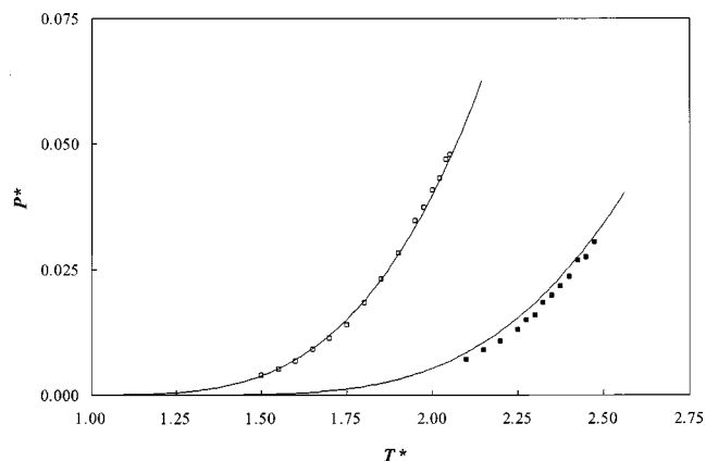
FIG. 2. Vapor pressure curve ( P^* - T^* representation) for 3CLJ and 5CLJ model systems with tangent segments from computer simulation (symbols) and predictions from Wertheim's TPT1 (curves). The open squares correspond to the simulations of this work for the rigid 3CLJ system, and the closed squares to those of the 5CLJ. The curves indicate the pressures as calculated with Wertheim's TPT1, which serves as a model for flexible systems.
