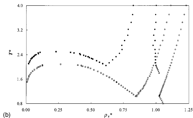
FIG. 4. Global phase diagram in (a) T^* - \rho^* and (b) T^* - \rho_s^* (where \rho_s^* = \rho^* m ) representations for linear rigid chain molecules of three and five tangent LJ segments as obtained from the simulations of this work. The open symbols correspond to the 3CLJ system and the closed symbols to the 5CLJ system. The squares correspond to the results of GEMC calculations, the triangles to the NPT calculations of the liquid phase at zero pressure, the circles to the solid-fluid coexistence densities obtained with Gibbs–Duhem calculations, and the asterisks and crosses to the solid densities obtained with NPT calculations at zero pressure.
