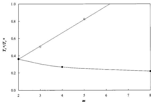
FIG. 7. Sketch of the T_t/T_c ratio for varying chain length in model chains of tangent LJ segments. The open symbols correspond to the ratios for linear rigid molecules as obtained in this work, and the closed symbols to the ratios of flexible molecules as obtained with Wertheim's TPT1 in previous work (Ref. 37). The curves are guides to the eye.
