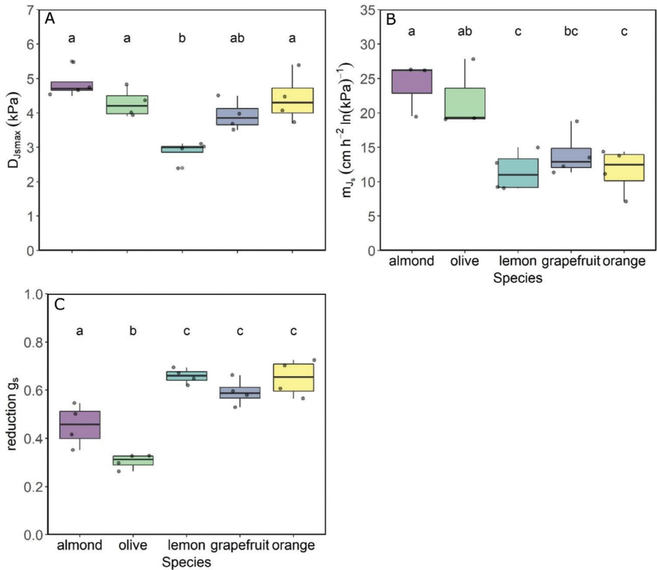
Fig. 2. Boxplot of (A) the vapour pressure deficit at which maximum sap flux density occurs ( D_{J_{smax}} ), (B) sensitivity of sap flux density ( J_s ) to vapour pressure deficit ( D ) ( m_{J_s} = dJ_s/d\ln D ), and (C) reduction of stomatal conductance ( g_s ) at D_{J_{smax}} compared with its maximum, calculated from data of the instrumented trees ( n=4 ) over the three measurement days.
