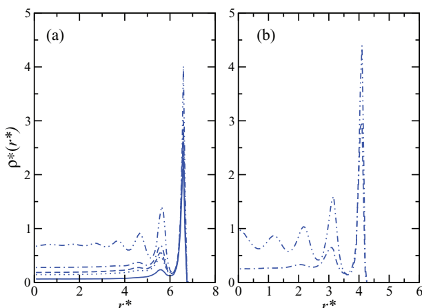
FIG. 1. Density profiles of LJ molecules adsorbed on cylindrical pores with pore radius (a) R^* = 7.5 and (b) R^* = 5.0 at T^* = 2.0 obtained from MC NVT simulations. The curves correspond to total densities inside the cylindrical pore of \rho^* = 0.1886 (continuous line), 0.2829 (dotted line), 0.3215 (dashed line), 0.3773 (dotted-dashed line), and 0.6431 (dotted-dotted-dashed line).
