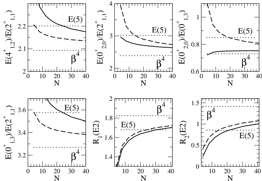
FIG. 2: Variation with the number of bosons (up to N = 40 ) of selected energy and B(E2) ratios for IBM calculations performed at the critical points of Hamiltonians (1) (broken line) and (2) (full line). The corresponding E(5) and \beta^4 values are marked with horizontal dotted lines.
