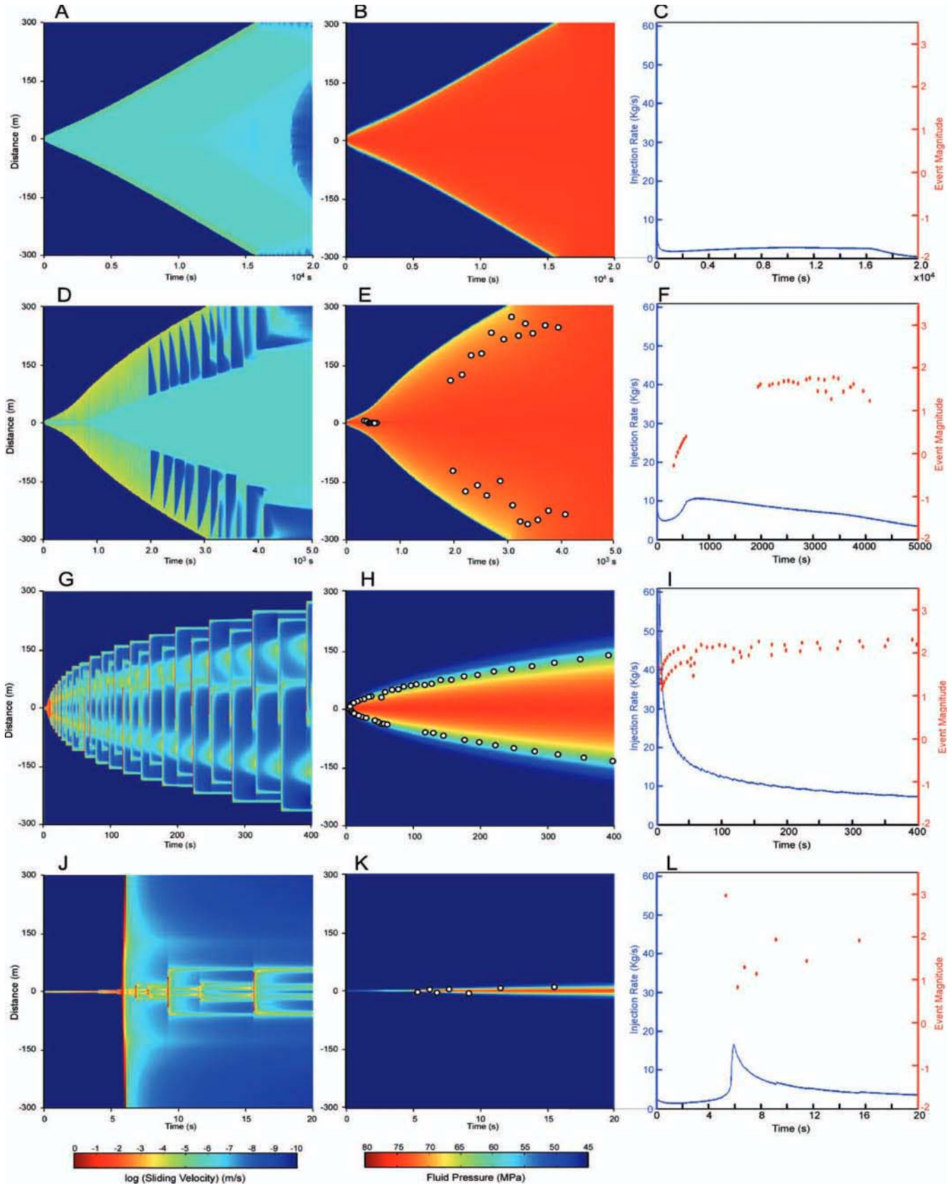
Fig 1. Sliding velocity (m/s), fluid pressure (MPa), injection rate (kg/s) and event magnitude evolution along fracture distance and time elapsed (s) for model \theta = 88^\circ (A-C), \theta = 86^\circ (D-F), \theta = 76^\circ (G-I) and \theta = 60^\circ (J-L). White points indicate hypocentre of seismic events. See color figure in the web.
