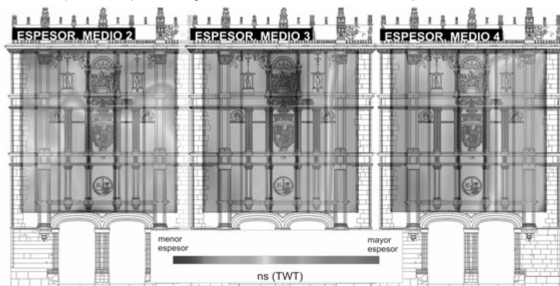
Fig. 4.- Results obtained from the lateral correlation of thickness variations of the units identified in the GPR profiles. See color figure in the web.
