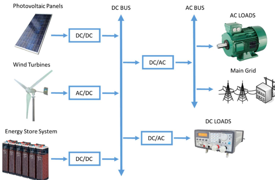
Fig. 5. Example of Hybrid bus.
