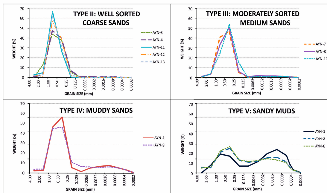
Figure 4. Types of grain size distribution within the (A) inner (fluvial) and (B) outer (marine) studied areas.
