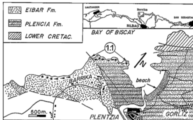
Fig. 1.—Geographic and geologic location of the Plentzia and Eibar Fm. outcrops in the neighbourhoods of Plentzia and Barrika towns. Upper figure for a more general situation.
