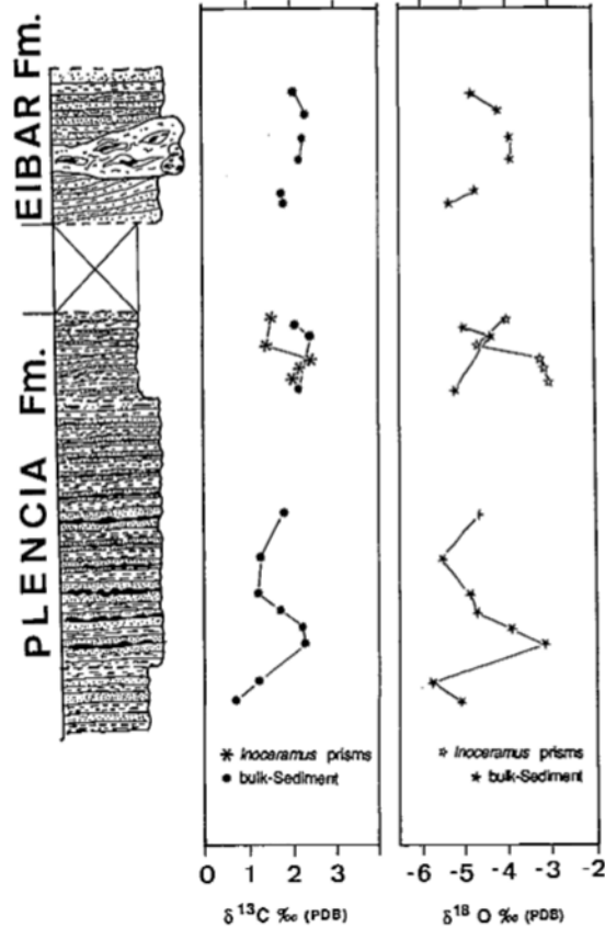
Fig. 4.—Carbon and oxygen stable-isotopic distribution of carbonate turbidites, Inoceramus prisms, siliciclastic turbidites (sandy flysch) plotted against the lithostratigraphy of the Plentzia and Eibar Fms.
