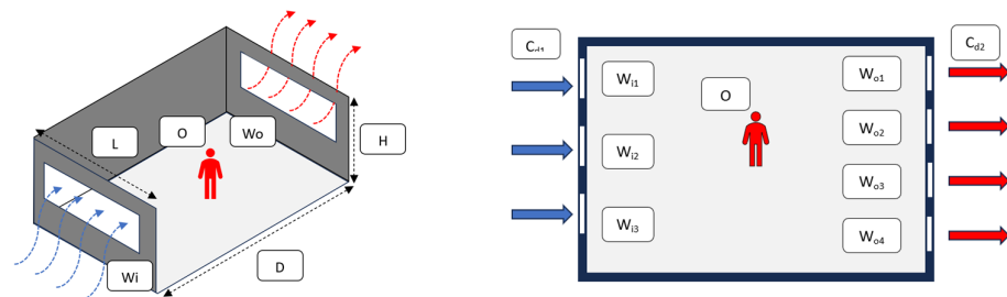
Figure 1. Main parameters affecting cross ventilation.
