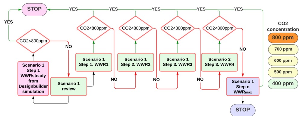
Figure 5. SNVP for optimal IAQ during winter season.
