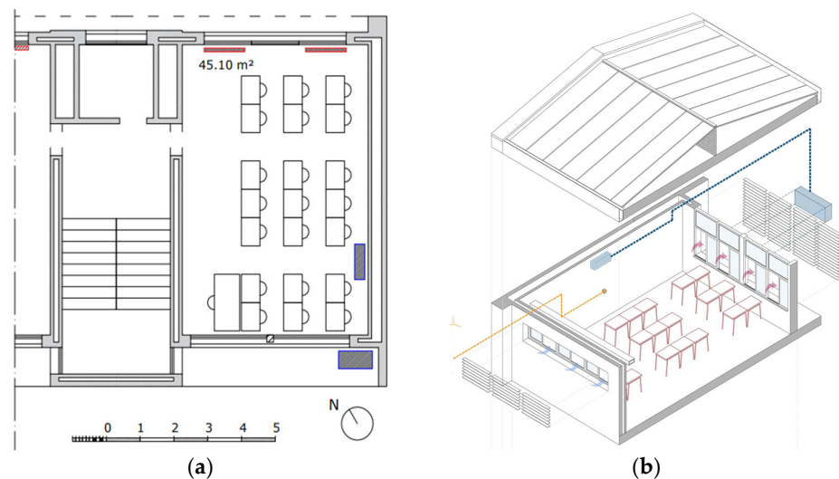
Figure 3. Classroom layout (a) and north 3D axonometric view of classroom (b).
