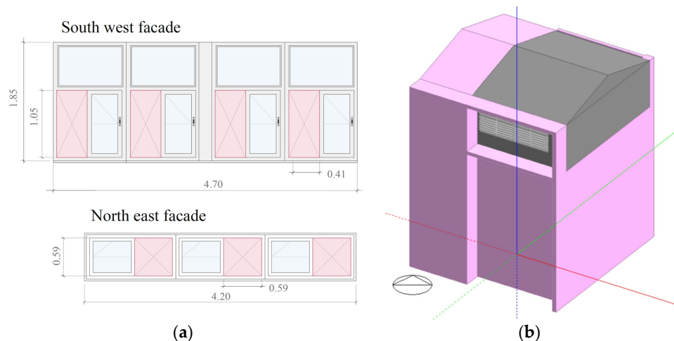
Figure 4. Opening elevation layout (a) and DesignBuilder TM model 3D view (b).
