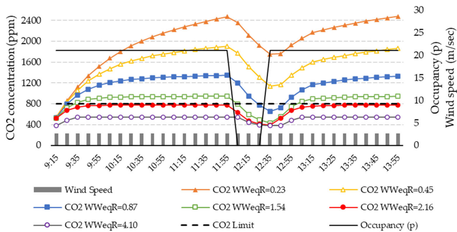
Figure 7. CO 2 concentration for different WWeqRs with SNVP.
