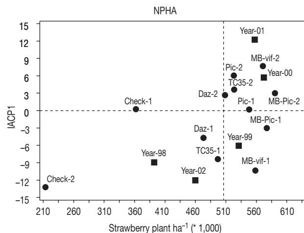
Figure 1. Biplot of principal component analysis (IPCA1) axis 1 against strawberry plant \text{ha}^{-1} for (●) methyl bromide alternatives in strawberry nurseries at (■) five years. The vertical line is the grand mean of the experiment. Treatment-1: «Viveros California» nursery. Treatment-2: «Viveros Rio Eresma» nursery.
