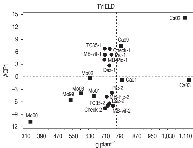
Figure 2. Biplot of principal component analysis (IPCA1) axis 1 against total yield for (●) MB alternatives in strawberry nurseries in (■) nine agro-environments (not including Ca00). The vertical line is the grand mean of the experiment. Treatment-1: «Viveros California» nursery. Treatment-2: «Viveros Rio Eresma» nursery.
