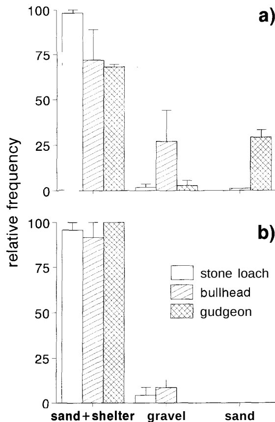
FIGURE 1. Mean relative frequency of the three kinds of substrata use by a) single species (allopatrically) and b) mixed species group (sympatrically). Error bars: \pm 1 SE.
