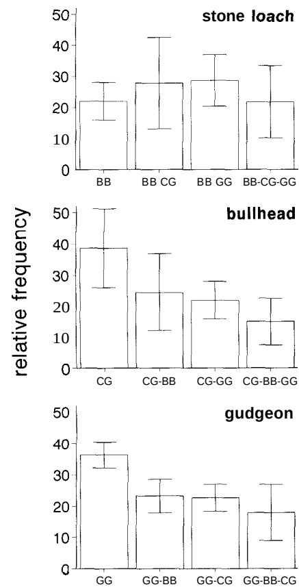
FIGURE 2. Mean relative frequency of species combinations under sheltered positions. Error bars: \pm 1 SE. BB: B. barbatula , CG: C. gobio , GG: G. gobio .
