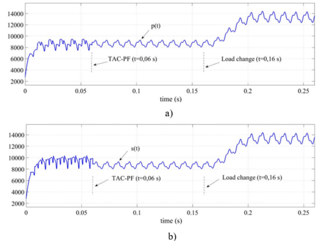
FIGURE 10. a) Instantaneous power (W) before/after TAC_PF ( t=0.06 s); b) Instantaneous apparent power (VA) before/after TAC_PF ( t=0.06 s). At t=0.16 s there is a change in the load.
