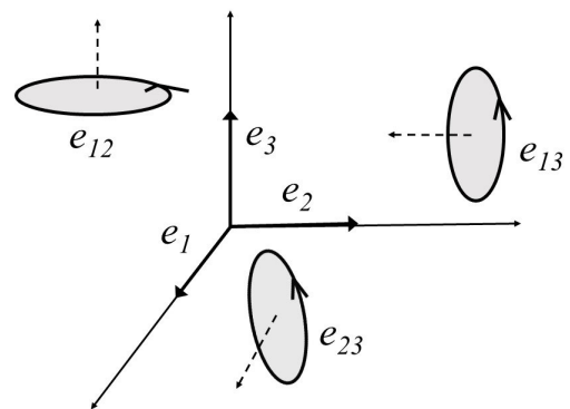
FIGURE 1. Basis vectors ( e_1, e_2, e_3 ) and basis bivectors ( e_{12}, e_{23}, e_{13} ) in three-dimensional Euclidean space.
