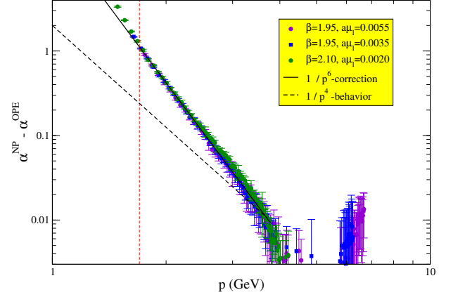
FIG. 1: The departure of lattice data from the leading non-perturbative OPE prediction for the running coupling plotted in logarithmic scales, in terms of the momentum manifestly shows a next-to-leading 1/p^6 behaviour; the dashed red line stands for the momentum scale, p \simeq 1.7 GeV, below which the lattice data do not follow the 1/p^6 behaviour any longer.
