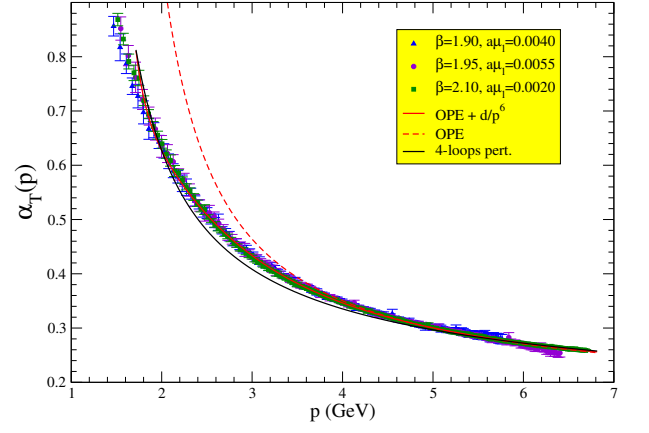
FIG. 3: Eq. (2) (red dashed) and Eq. (3) (red solid) for the parameters in Tab. I fitted to the lattice data for \alpha_T defined by (1). The black line is for Eq. (2) with g^2\langle A^2 \rangle = 0 .
