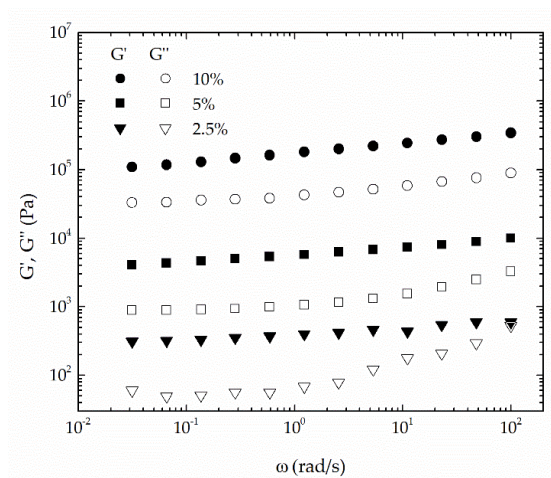
Figure 5. Evolution of the storage ( G' ) and loss ( G'' ) moduli with frequency for epoxidized lignin-based oleogels prepared with sample EAL1 at different concentrations ( G' , filled symbols; G'' , empty symbols).
