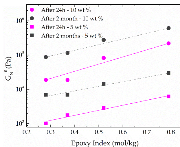
Figure 6. Evolution of G_N^0 with lignin epoxy index for EAL-based oleogels (5 and 10 wt % EAL) 24 h and 2 months after preparation.
