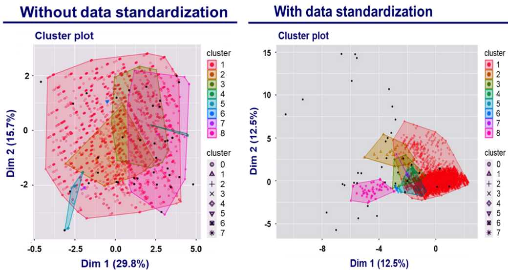
Figure 4. Visualization of the clusters
